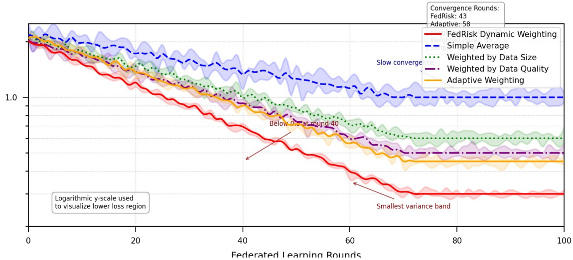
Fig. 3. Convergence Analysis of Parameter Aggregation Methods
