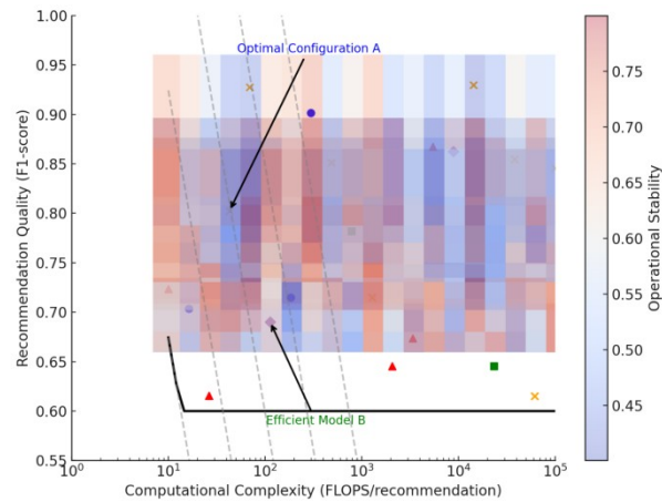
Figure 5. Pareto Frontier of Recommendation Accuracy vs. Computational Efficiency
