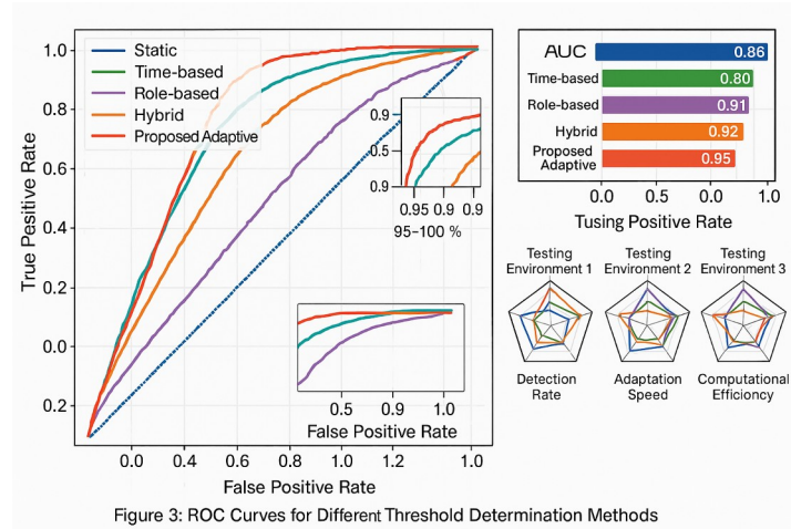
Figure 3: ROC Curves for Different Threshold Determination Methods
