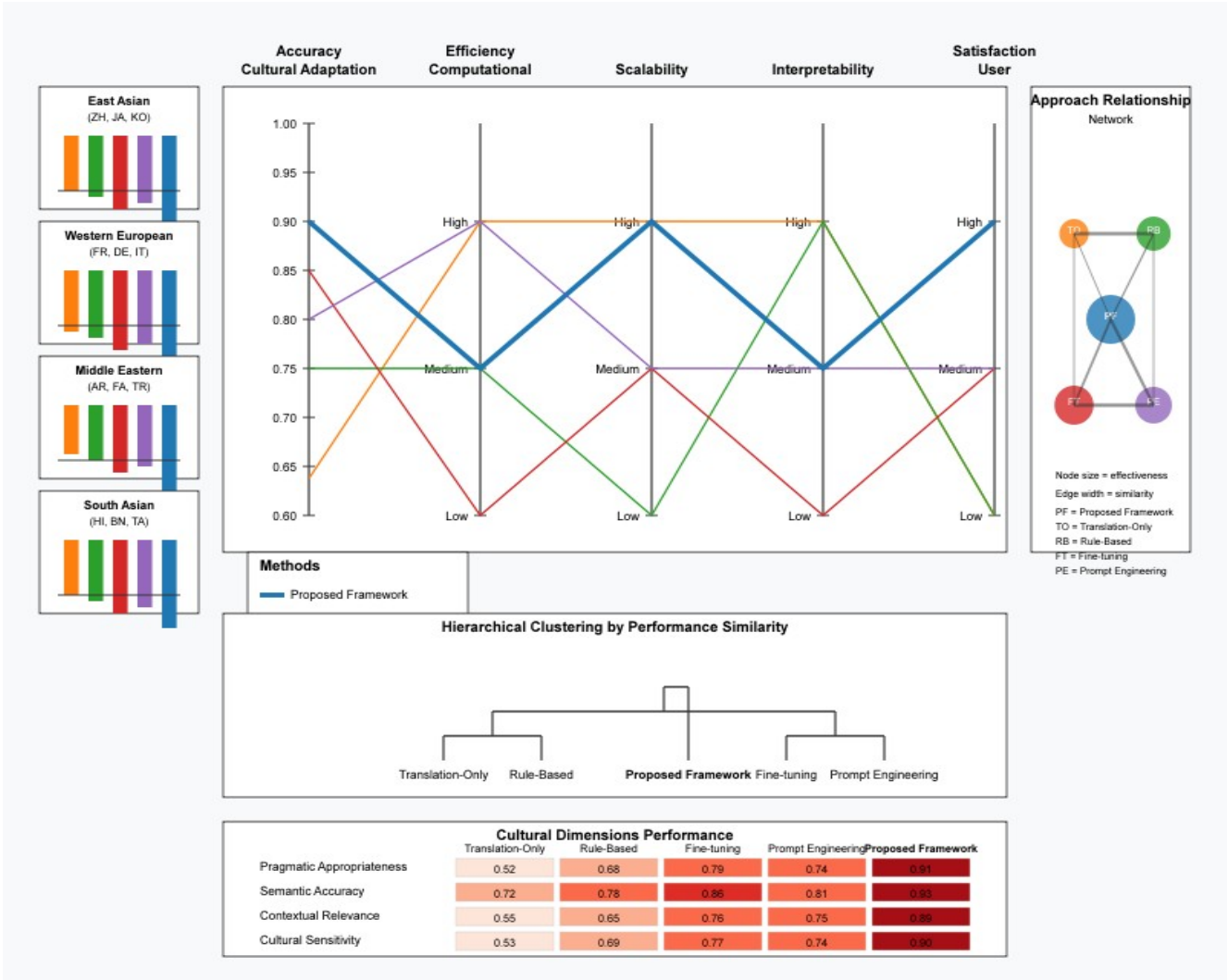
Figure 6: Multifaceted Comparative Analysis Visualization
