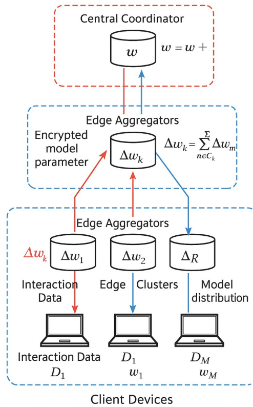
Figure 1: FedPrivRec System Architecture and Data Flow
