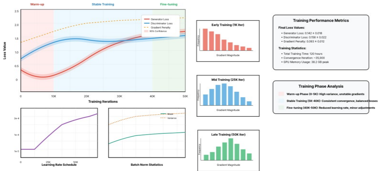
Figure 2: GAN Training Loss Convergence Analysis
