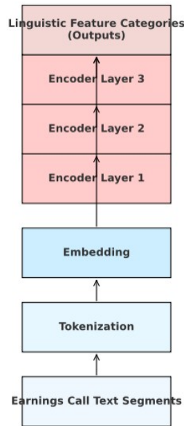
Figure 2: BERT-Based Linguistic Feature Extraction Architecture
