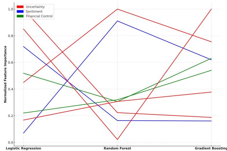
Figure 3: Feature Importance in Risk Prediction Models
