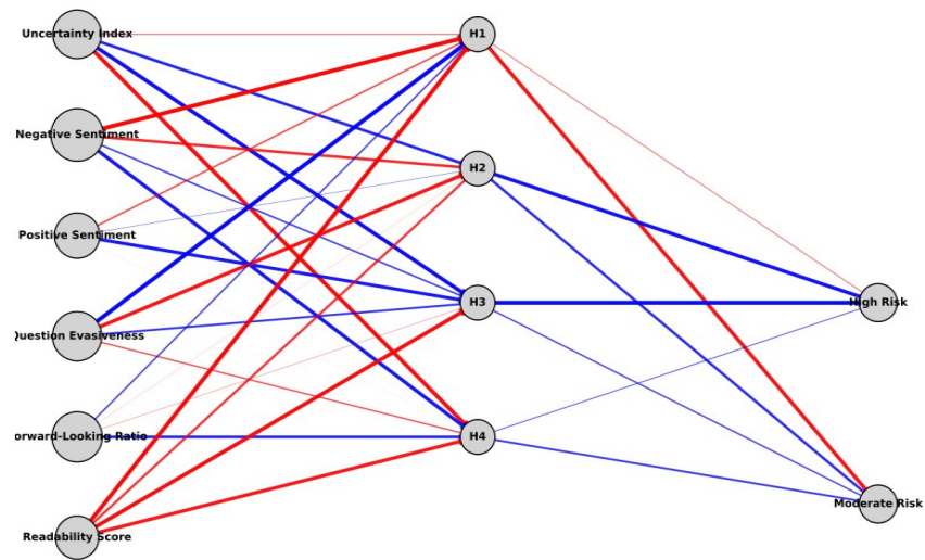
Figure 4: Neural Network Visualization of Linguistic Feature Relationships to Risk Events
