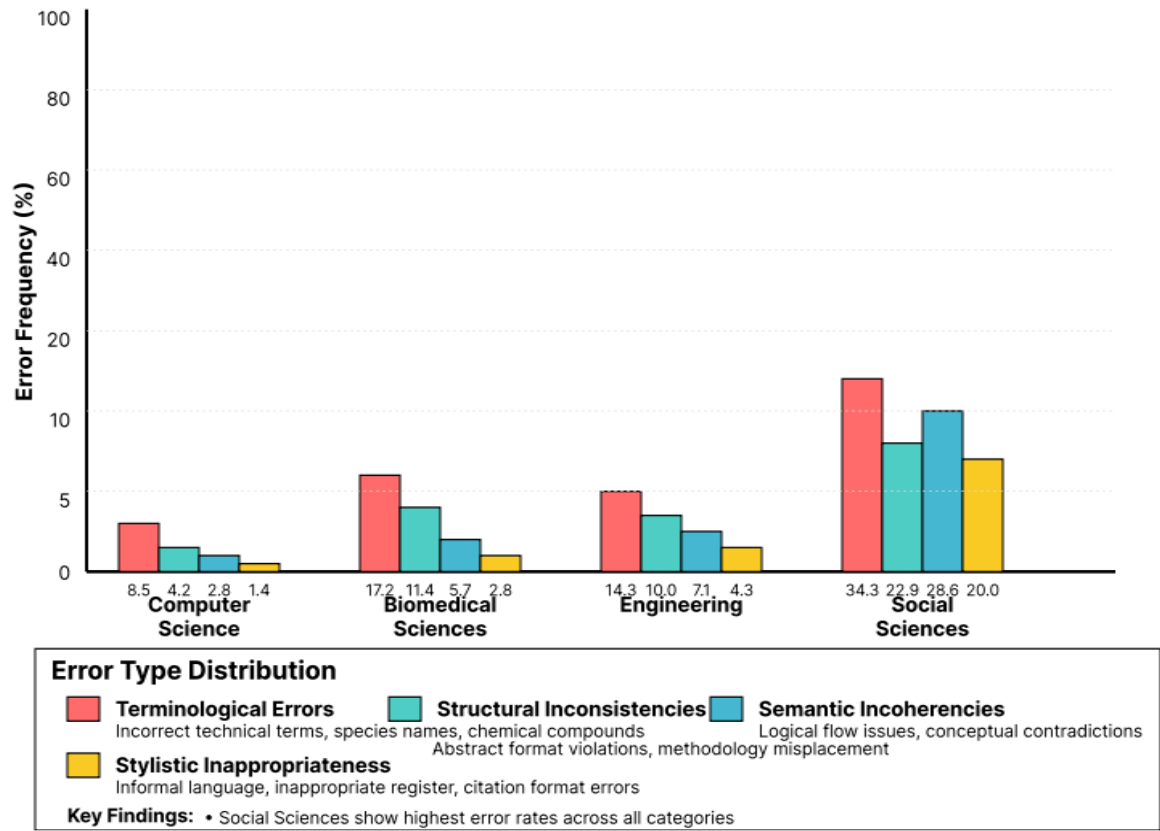
Figure 5: Error Pattern Analysis Across Domains
