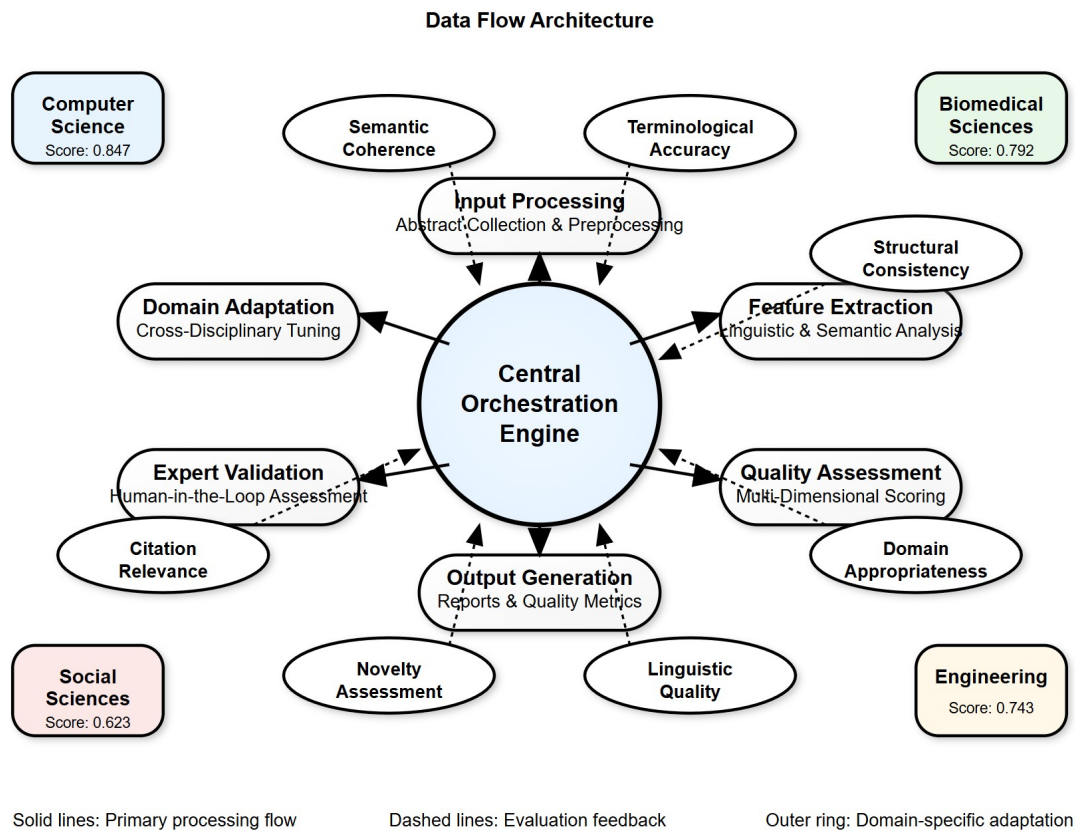
Figure 1: Multi-Dimensional Evaluation Framework Architecture
