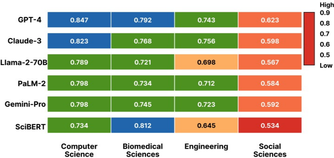
Figure 2: Domain Adaptation Performance Heatmap
