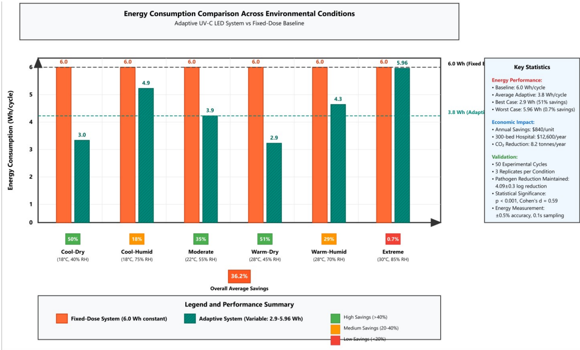
Fig. 3: Energy Consumption Comparison Across Environmental Conditions
