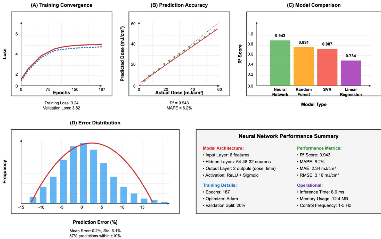
Fig. 2: Neural Network Training Convergence
