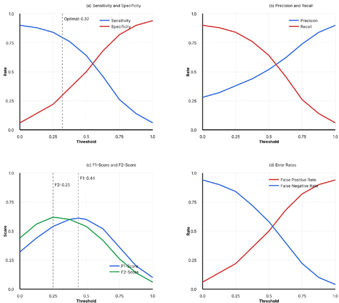
Figure 3: Threshold Sensitivity Analysis for Hybrid-GBM Combination
