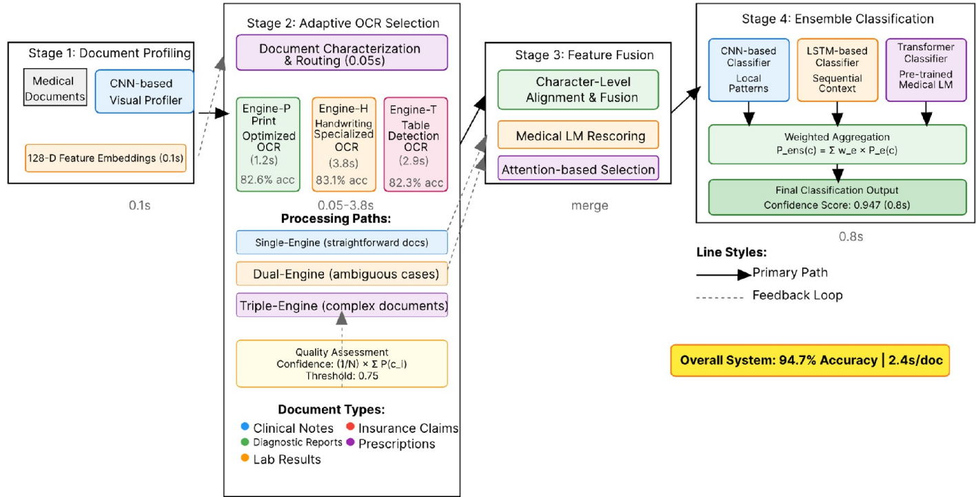
Figure 1: Multi-Engine Classification Framework Architecture
