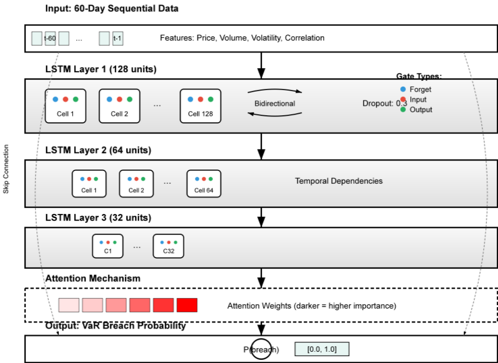
Figure 3: LSTM Architecture for VaR Prediction
