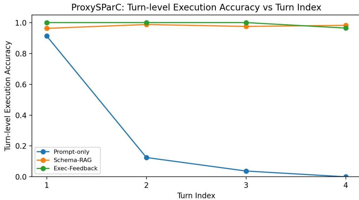
Fig. 4. ProxySPaC turn-level execution accuracy vs. turn index.
