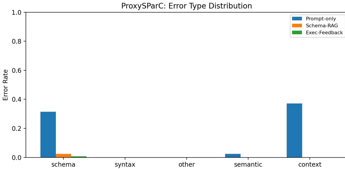
Fig. 8. ProxySPaRC error-type distribution (rates over all turns).
