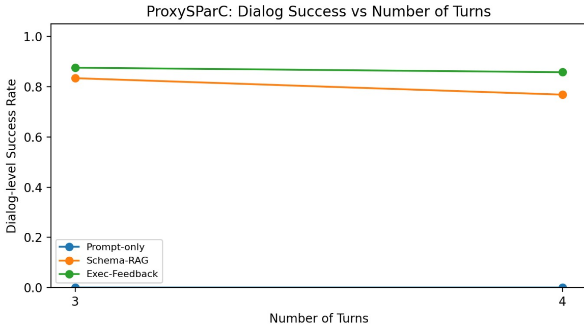
Fig. 6. ProxySPaRC dialog-level success vs. number of turns.
