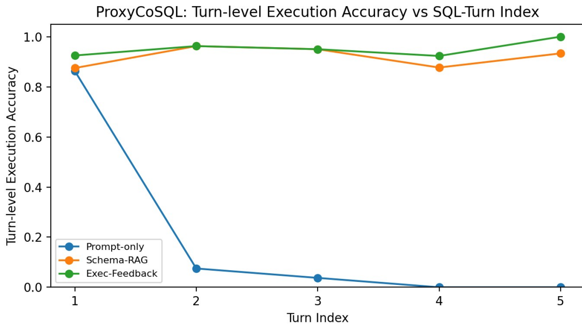
Fig. 5. ProxyCoSQL turn-level execution accuracy vs. SQL-turn index.
