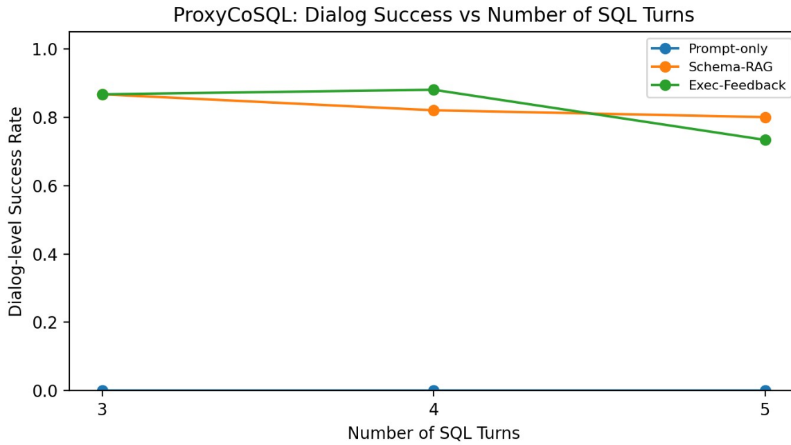
Fig. 7. ProxyCoSQL dialog-level success vs. number of SQL turns.
