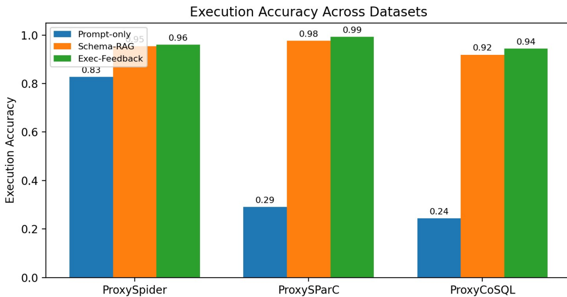
Fig. 3. Execution accuracy across datasets for the three paradigms.
