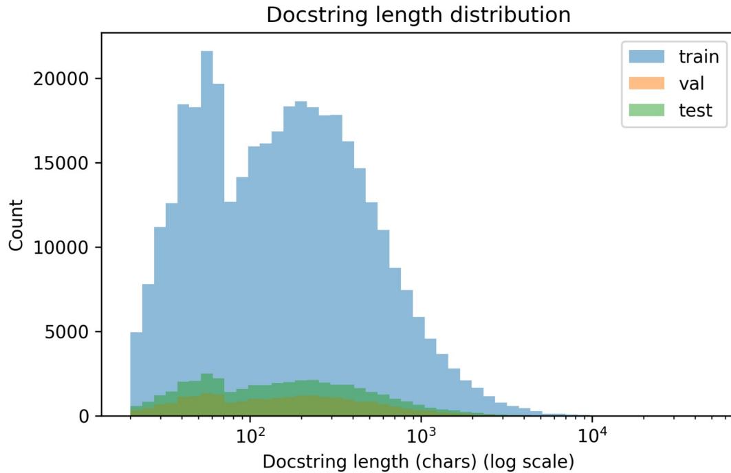
Fig. 3. Docstring length distributions across splits (log-scaled x-axis).
