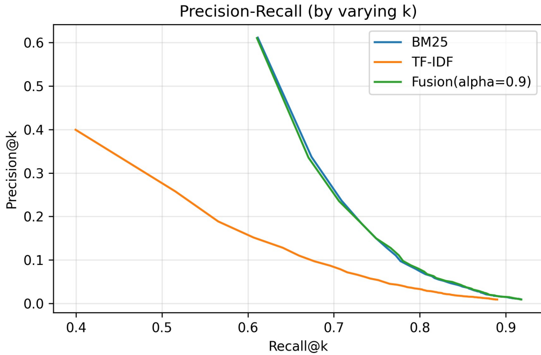
Fig. 5. Precision–Recall curves obtained by varying k (single relevant item per query).
