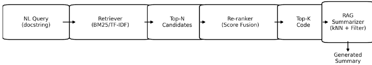
Fig. 1. Retrieval–summary integrated pipeline (“findable then explainable”).
