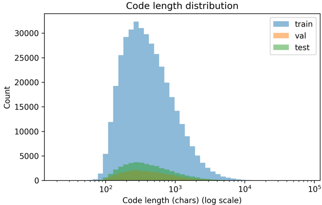
Fig. 2. Code length distributions across splits (log-scaled x-axis).
