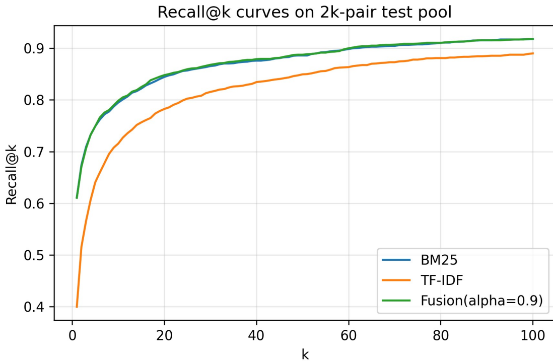
Fig. 4. Recall@k curves for retrieval methods (test pool, k=1 \dots 100 ).
