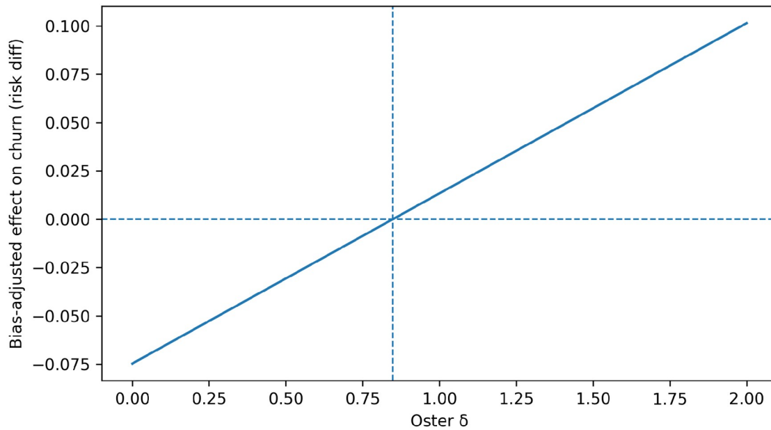
Figure 7. Oster sensitivity curve for churn ATE ( \delta on x-axis).
