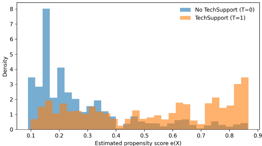
Figure 3. Propensity-score overlap for TechSupport treatment (logistic regression).
