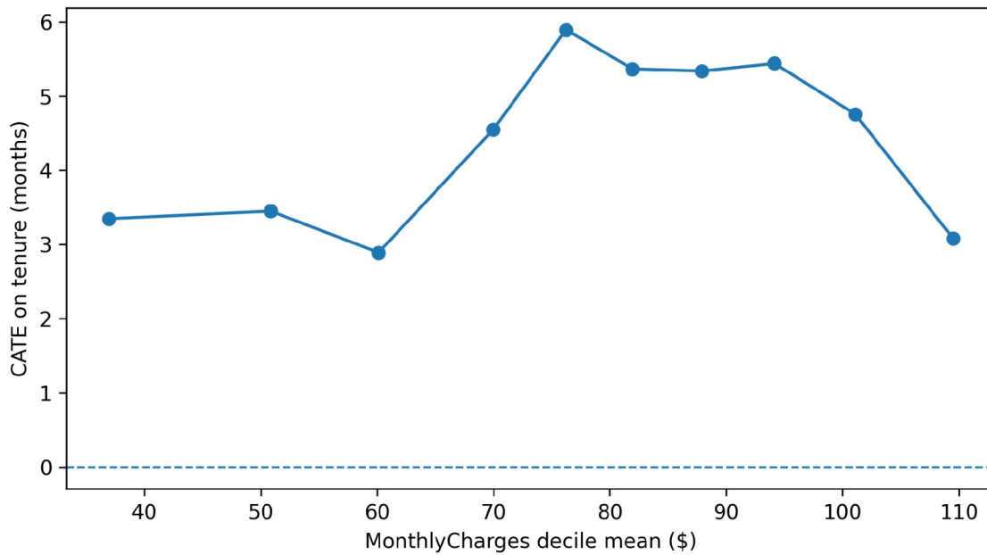
Figure 5. Tenure increment curve: CATE on tenure by MonthlyCharges segment.
