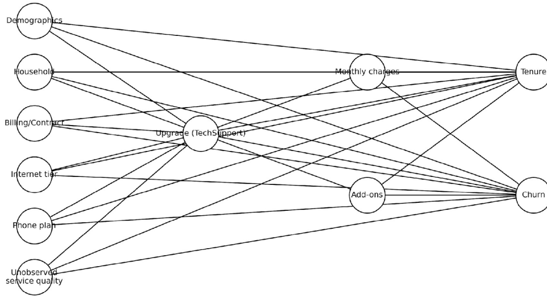
Figure 2. LLM-proposed DAG linking TechSupport upgrade to tenure and churn.
