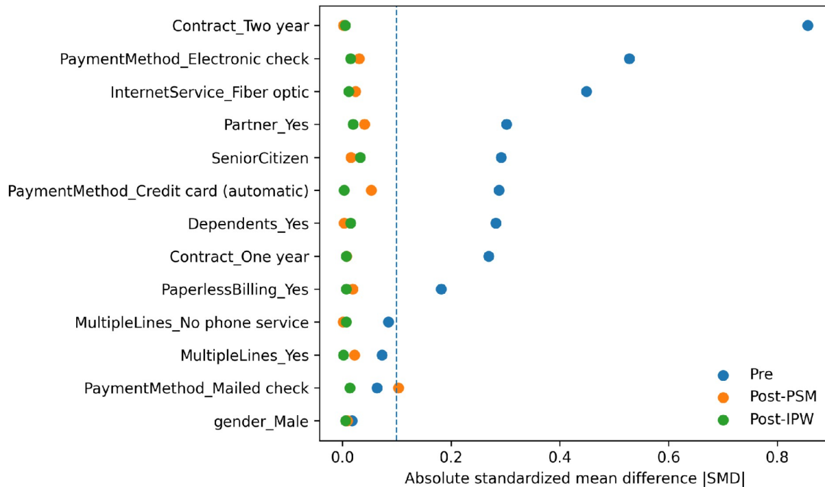
Figure 4. Love plot of absolute SMD before and after adjustment (PSM and IPW).
