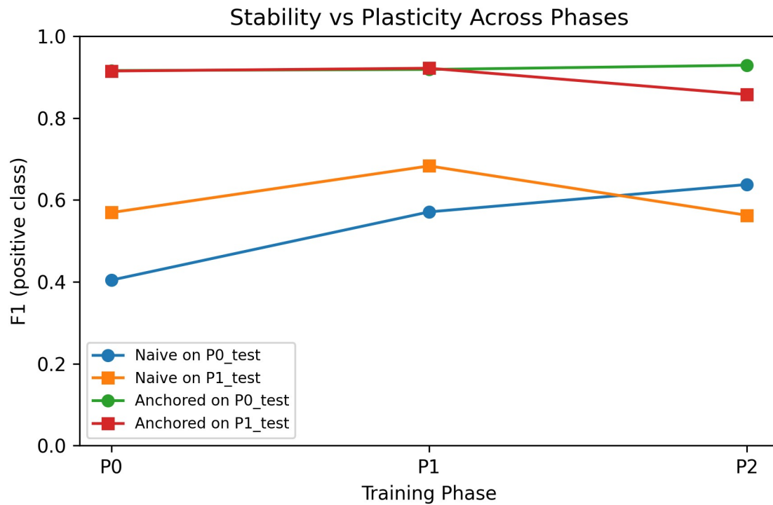
Figure 4. Stability–plasticity curves (F1 across phases) for naïve vs anchored online updates.
