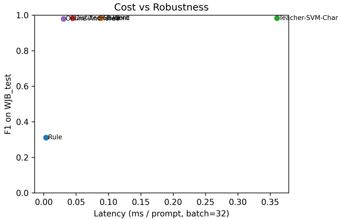
Figure 5. Cost vs robustness: latency (ms/prompt) versus F1 on WJB_test.
