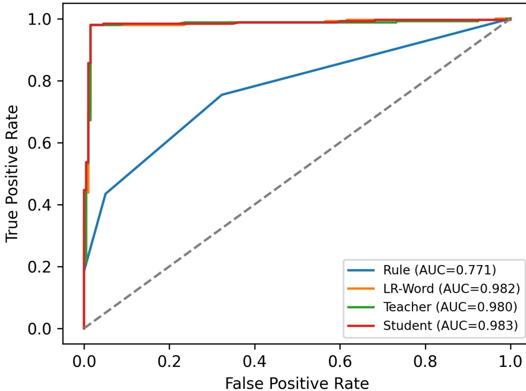
ROC on WJB_test (train=ITW)
