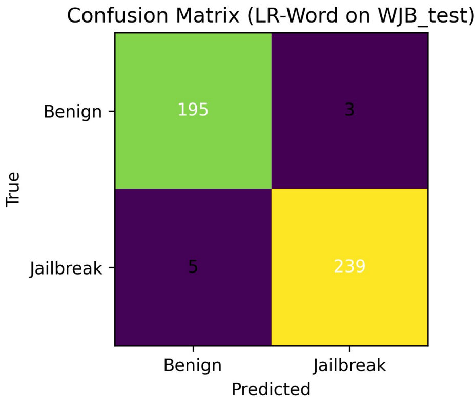
Figure 6. Confusion matrix for LR-Word (train=ITW) on WJB_test at \tau=0.5 .
