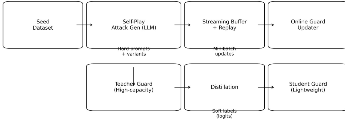
Figure 1. Continual red-teaming loop: self-play generation → streaming buffer → online update → teacher-to-student distillation.
