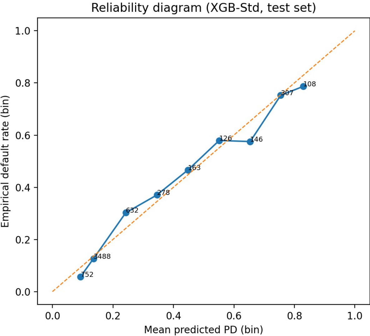
Fig. 6. Reliability diagram for XGB-Std on the test set (numbers denote bin counts).
