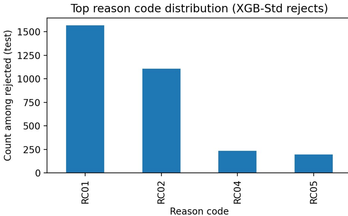
Fig. 7. Distribution of principal adverse-action reason codes among rejected applicants (XGB-Std under base policy).
