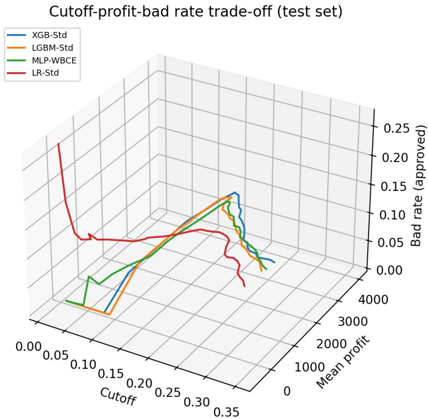
Fig. 5. Three-dimensional cutoff–profit–bad-rate trade-off curves (test set).
