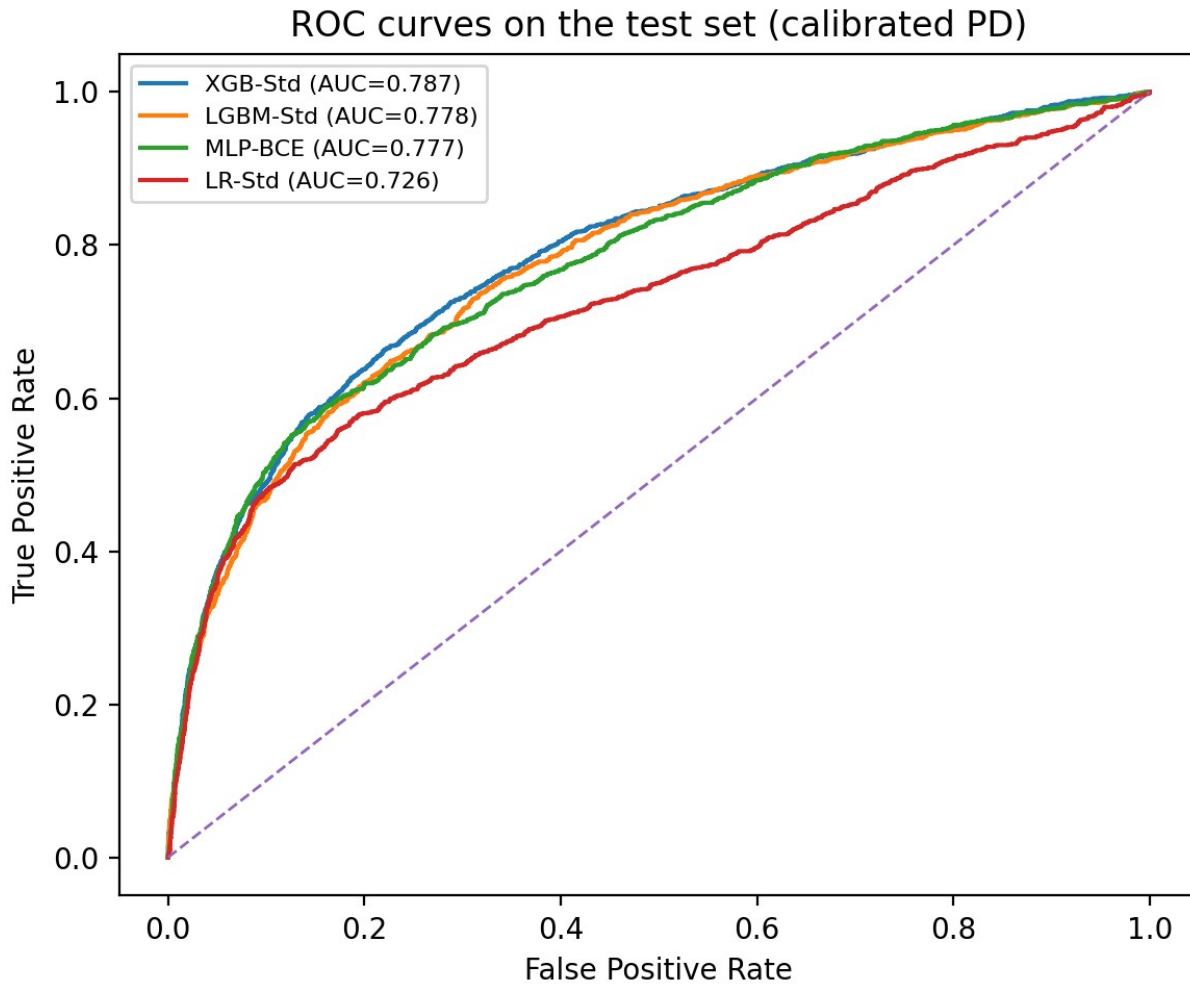
Fig. 3. ROC curves on the test set for representative models (calibrated PD).
