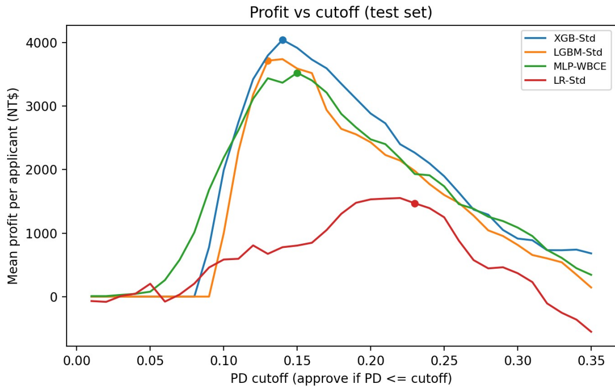
Fig. 4. Mean profit as a function of PD cutoff (test set). Markers indicate selected constrained profit-maximizing cutoffs.
