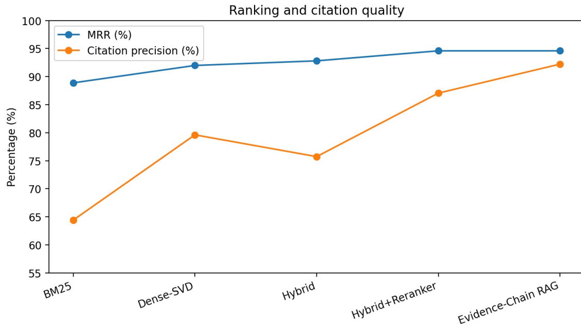
Figure 7. MRR and citation precision trend across the retrieval/RAG variants.
