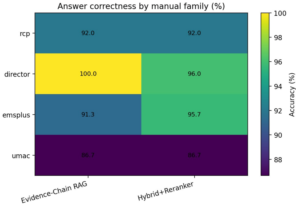
Figure 5. Per-family answer correctness for the two strongest grounded methods.
