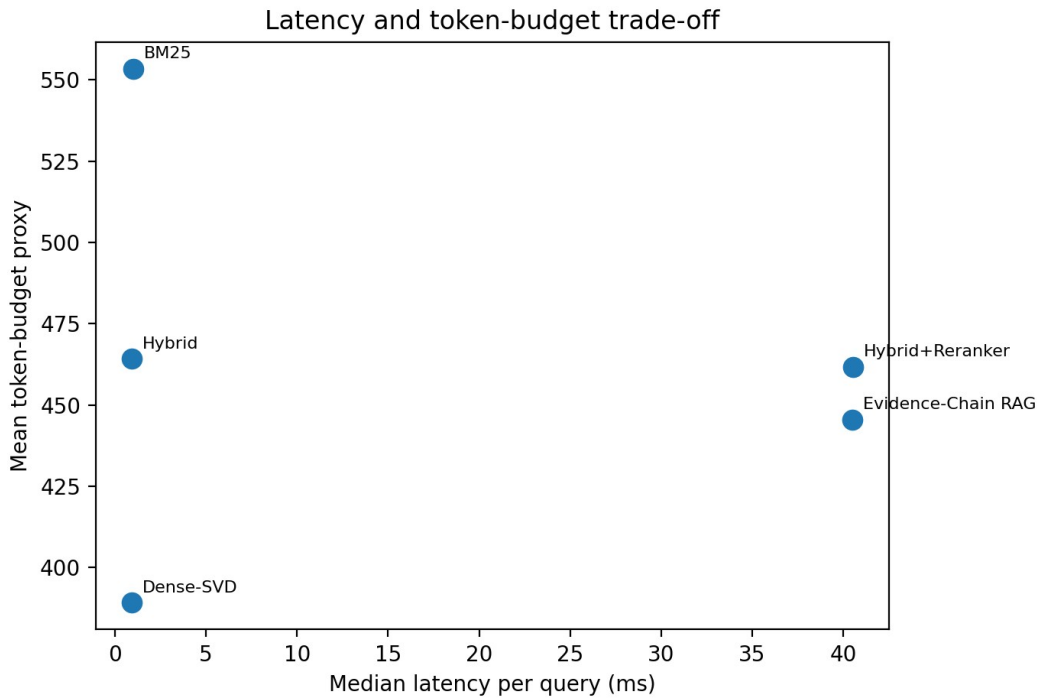
Figure 6. Latency and token-budget trade-off.
