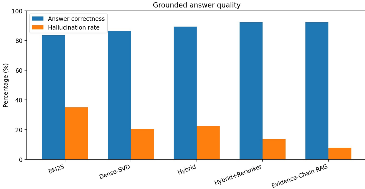
Figure 4. Answer correctness and hallucination rate by method.
