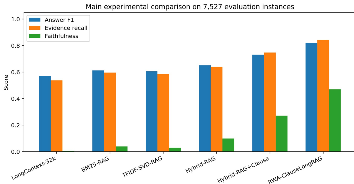
Figure 3. Main metric comparison for all evaluated systems.
