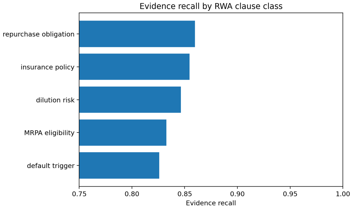
Figure 4. Clause-level evidence recall for RWA-ClauseLongRAG.
