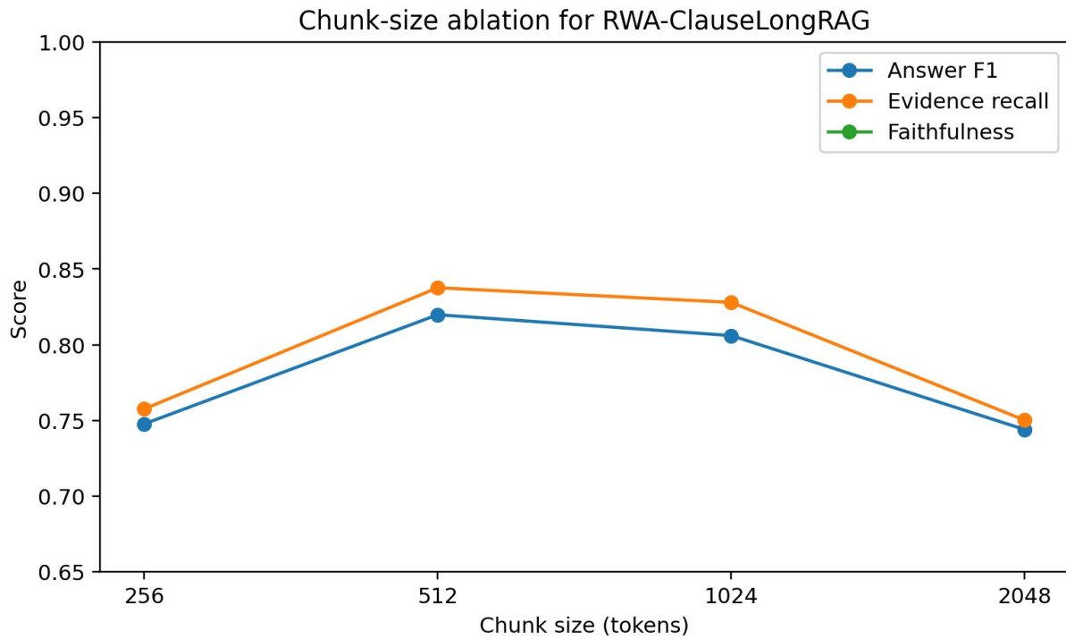
Figure 5. Chunk-size ablation: answer F1, evidence recall, faithfulness, and latency.
