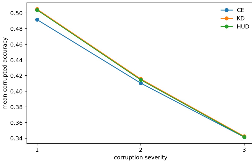
Fig. 6. Mean corrupted accuracy by severity for CE, KD, and HUD.
