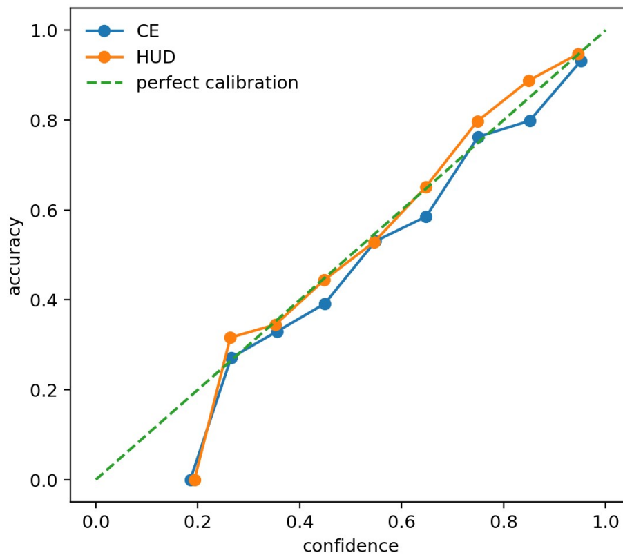
Fig. 4. Reliability diagram comparing CE and HUD on the test split.
