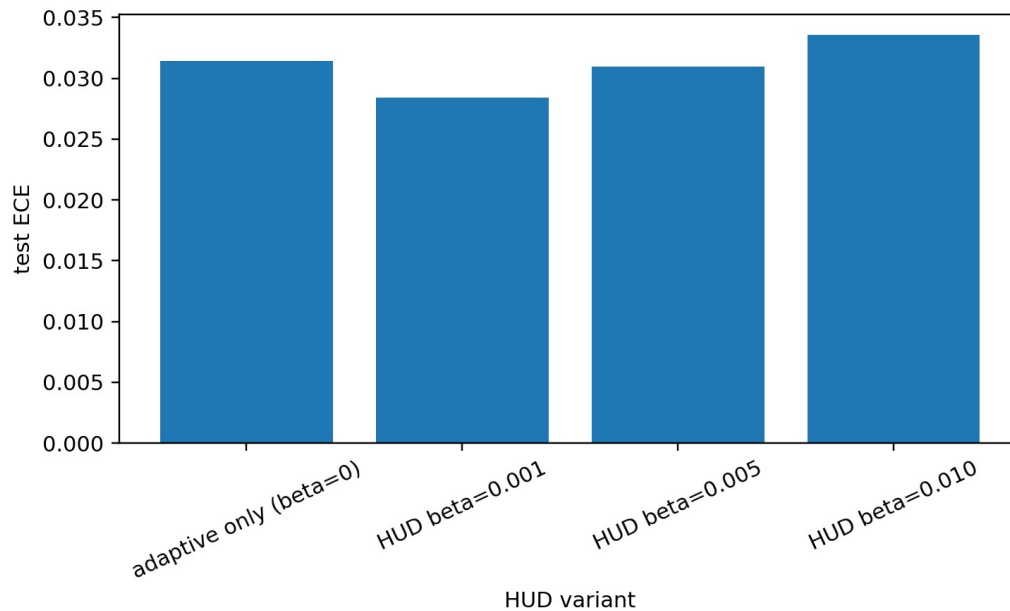
Fig. 8. Test ECE for the tested HUD variants.
