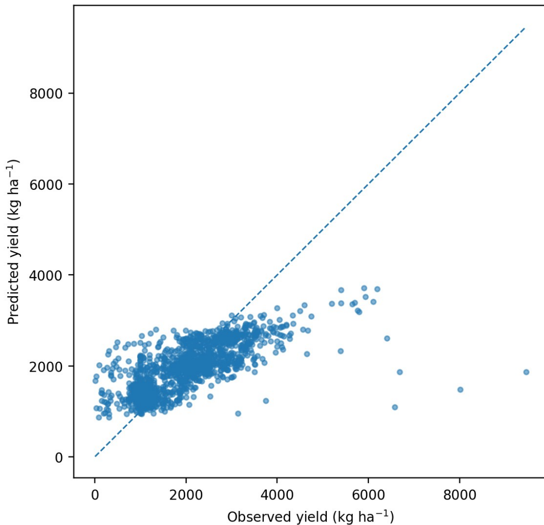
Figure 6. Observed versus predicted cereal yield for the best yield model.
