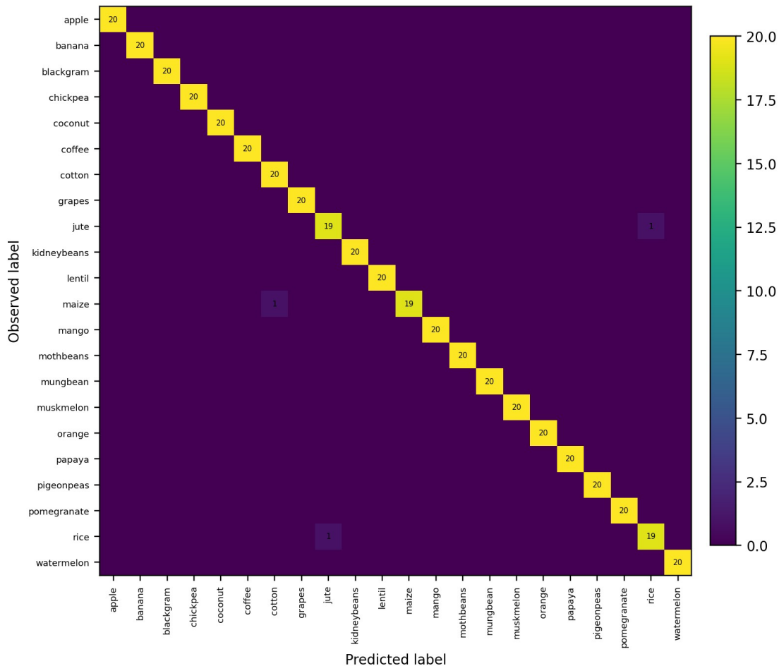
Figure 4. Confusion matrix of the best crop classifier.
