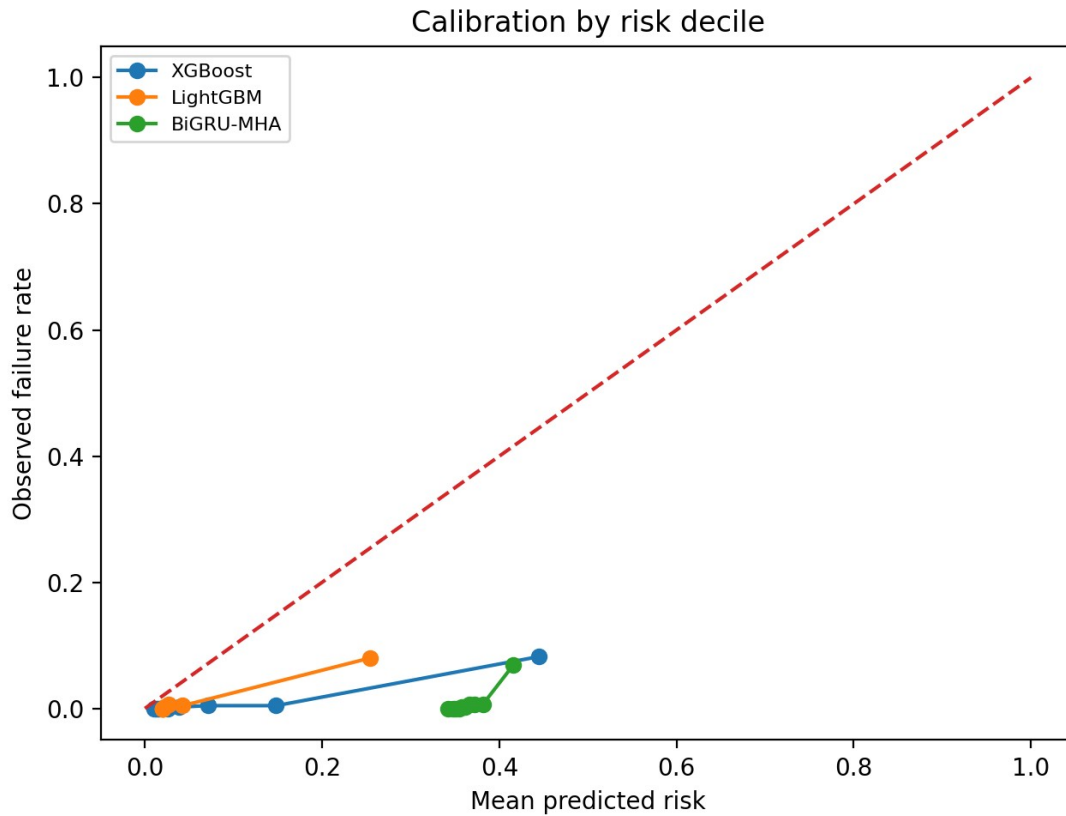
Figure 8. Calibration by predicted-risk decile.
