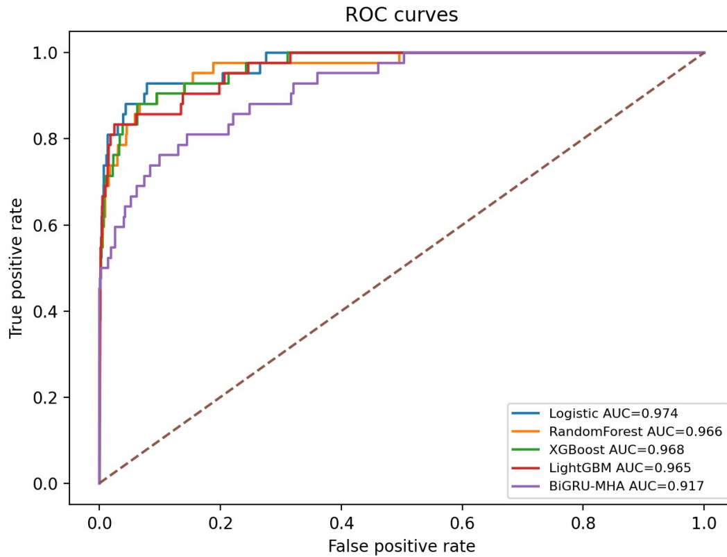
Figure 4. ROC curves on the held-out test split.
