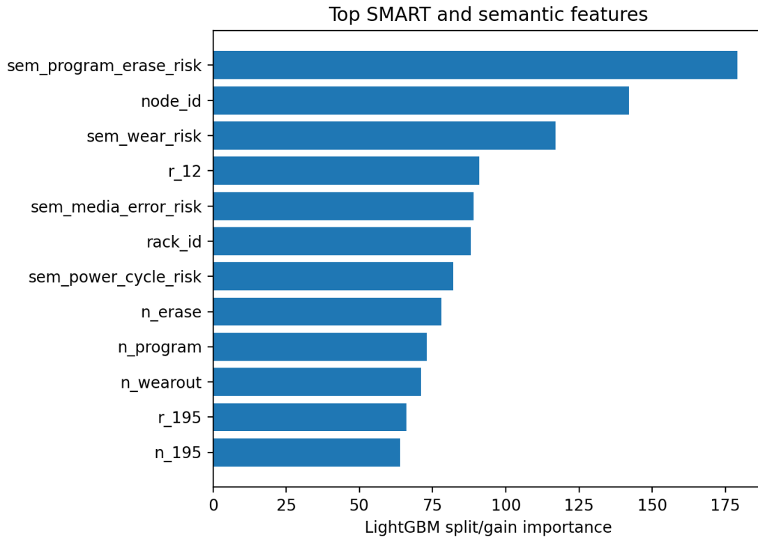
Figure 6. Leading SMART and semantic features by LightGBM importance.
