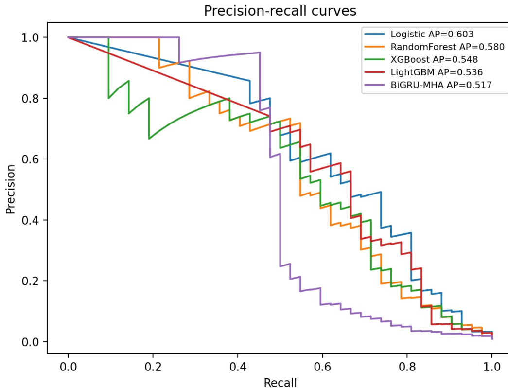
Figure 3. Precision-recall curves on the held-out test split.
