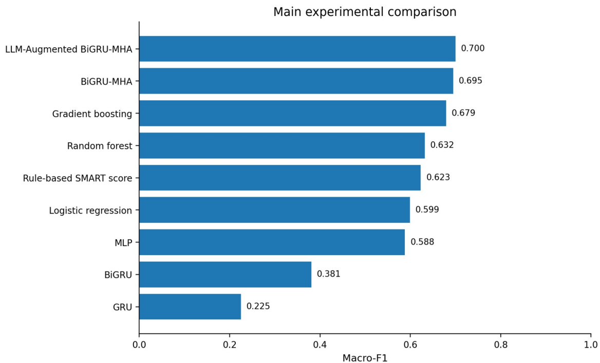
Figure 3. Macro-F1 comparison across classical and neural models.
