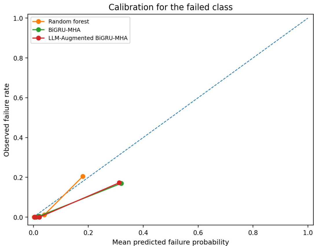
Figure 7. Failed-class calibration curve.
