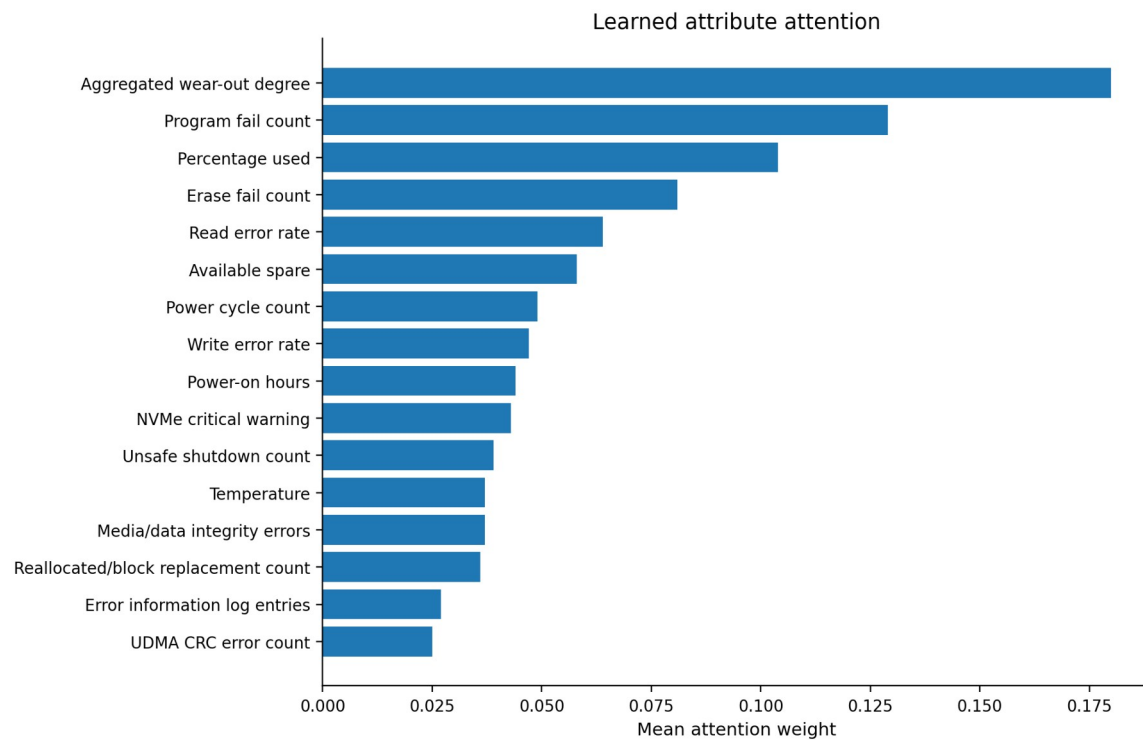
Figure 5. Attention-weight ranking for the 16 SMART attributes.
