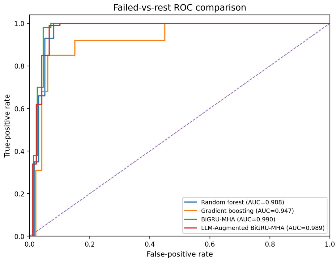
Figure 6. Failed-vs-rest ROC curves for selected models.
