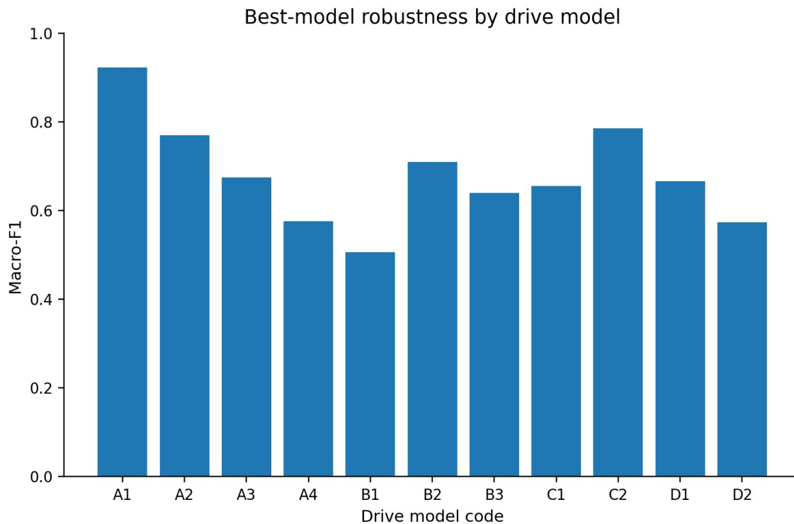
Figure 8. Macro-F1 by anonymized drive-model code.
