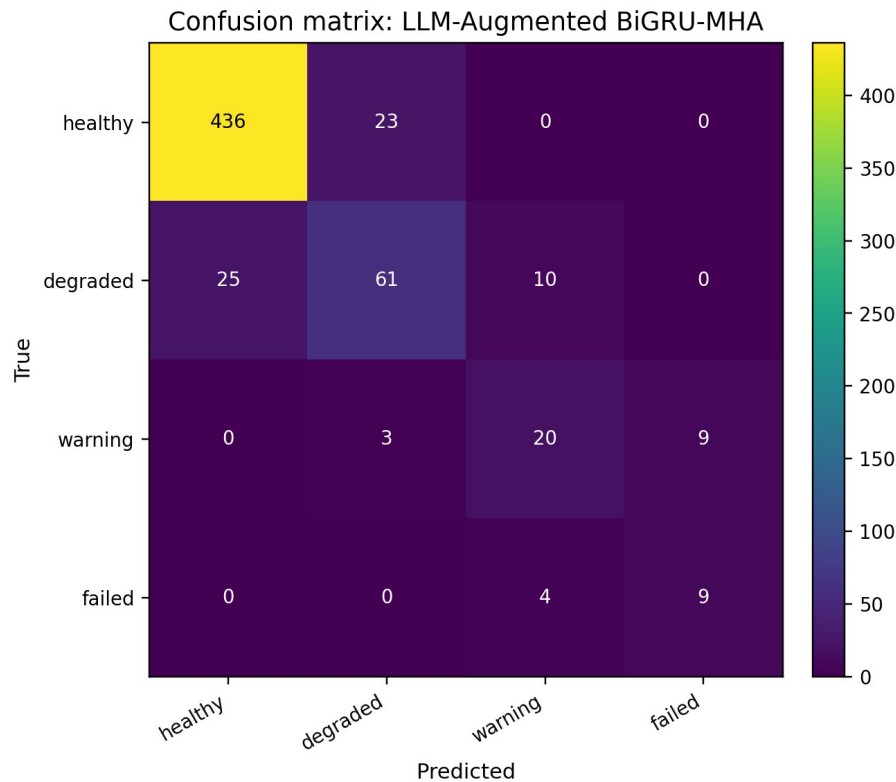
Figure 4. Confusion matrix of the proposed model.
