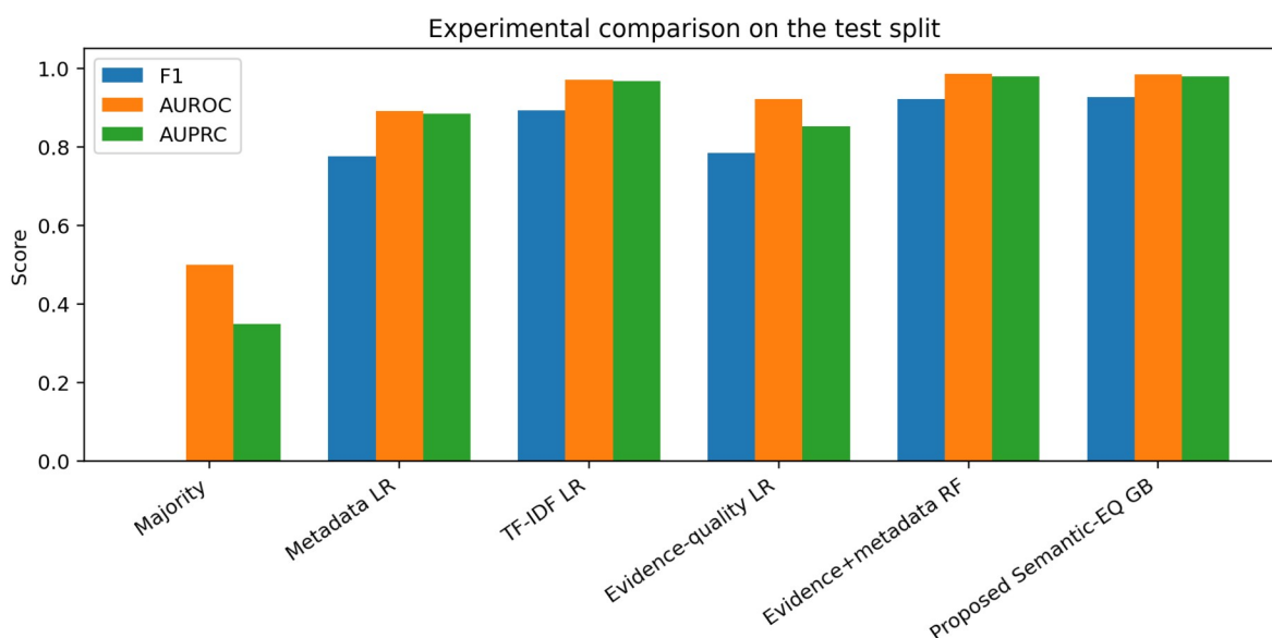
Figure 3. F1, AUROC, and AUPRC comparison across the tested methods.
