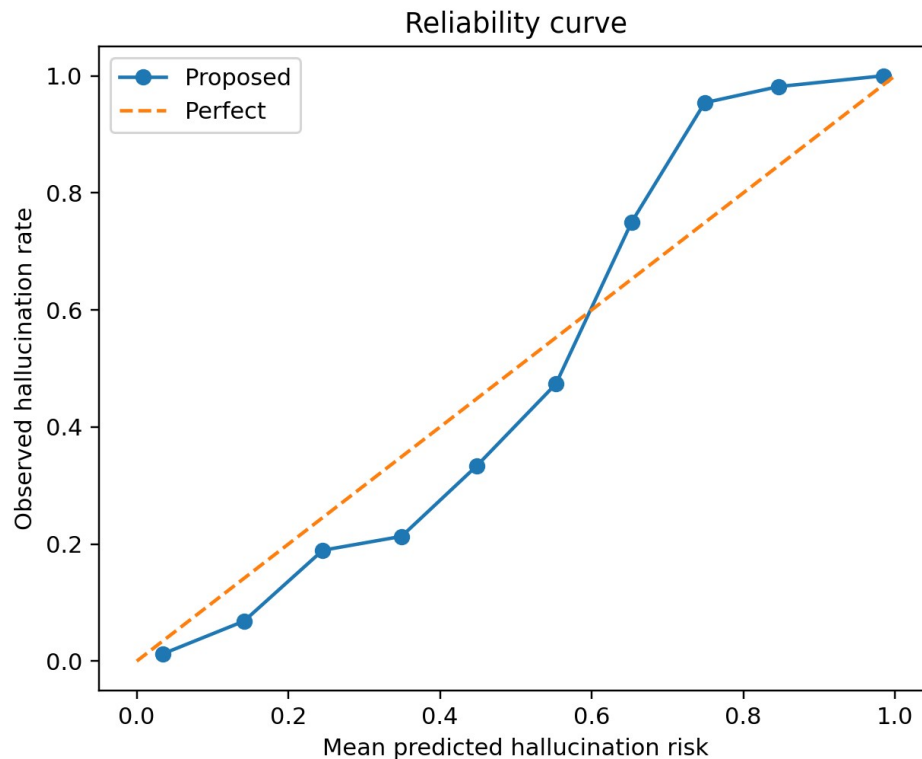
Figure 6. Reliability curve for the proposed hallucination-risk probabilities.
