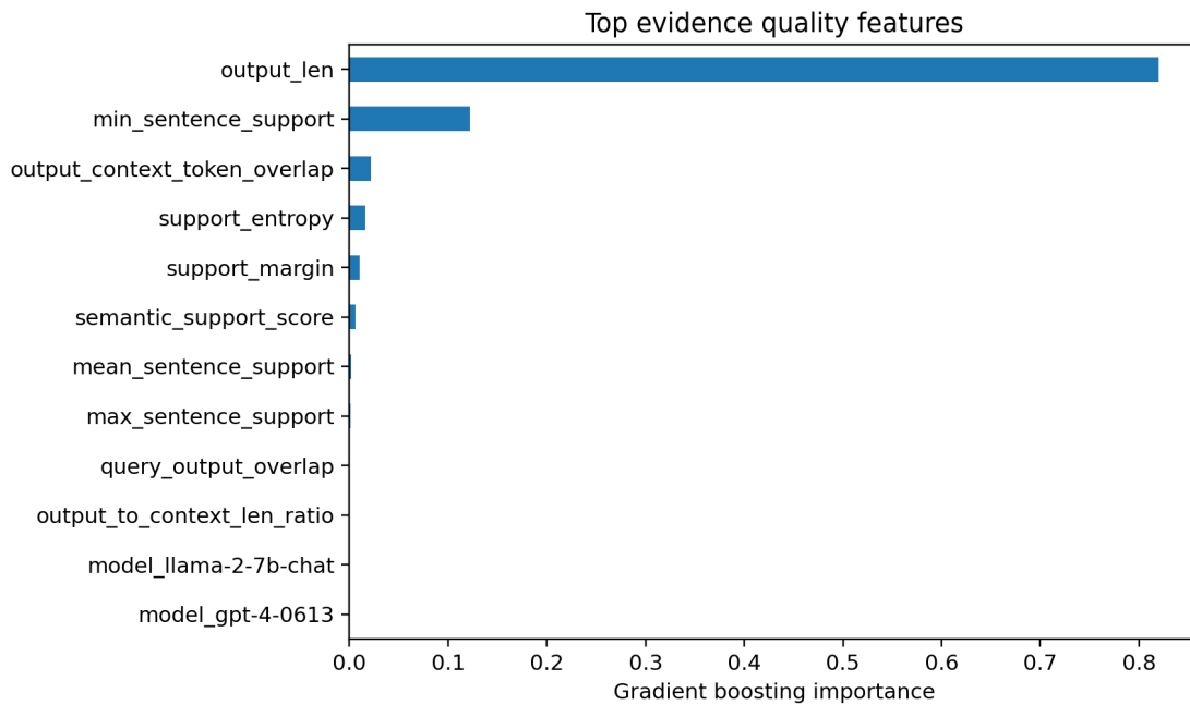
Figure 5. Top feature importances for the proposed gradient boosting model.
