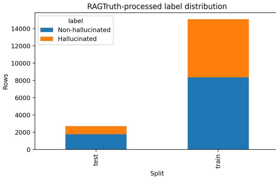
Figure 2. Train and test distribution of hallucinated and non-hallucinated outputs.
