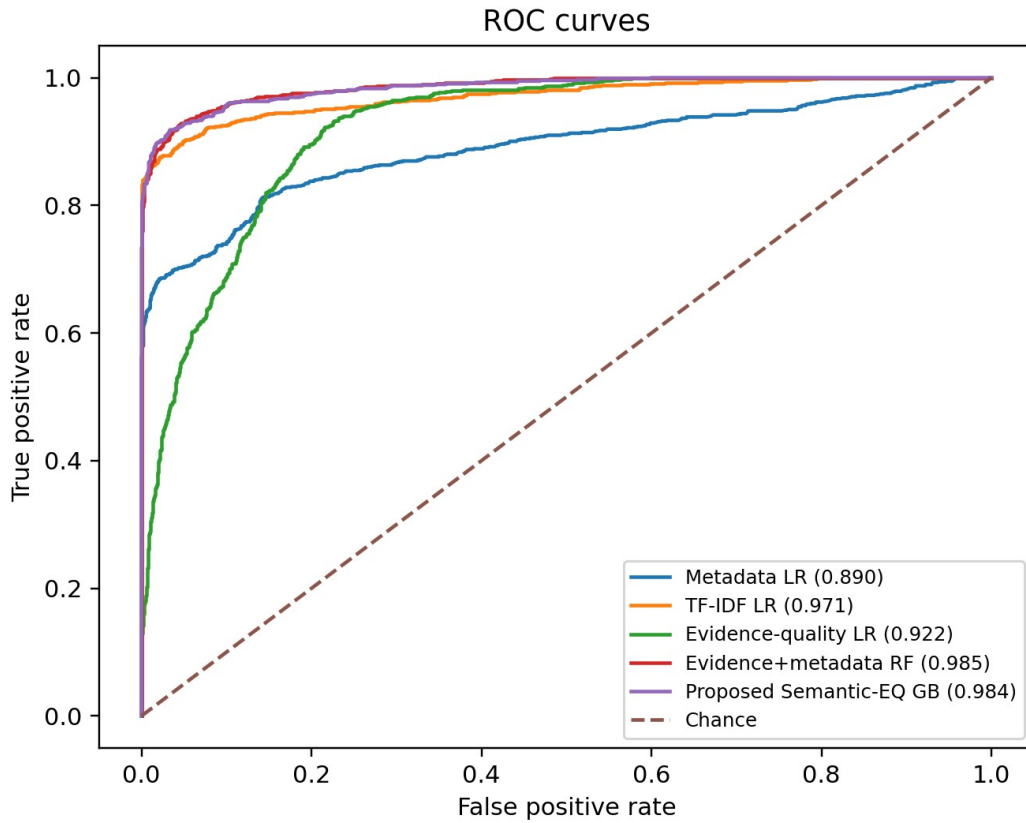
Figure 4. ROC curves for hallucination-risk ranking.
