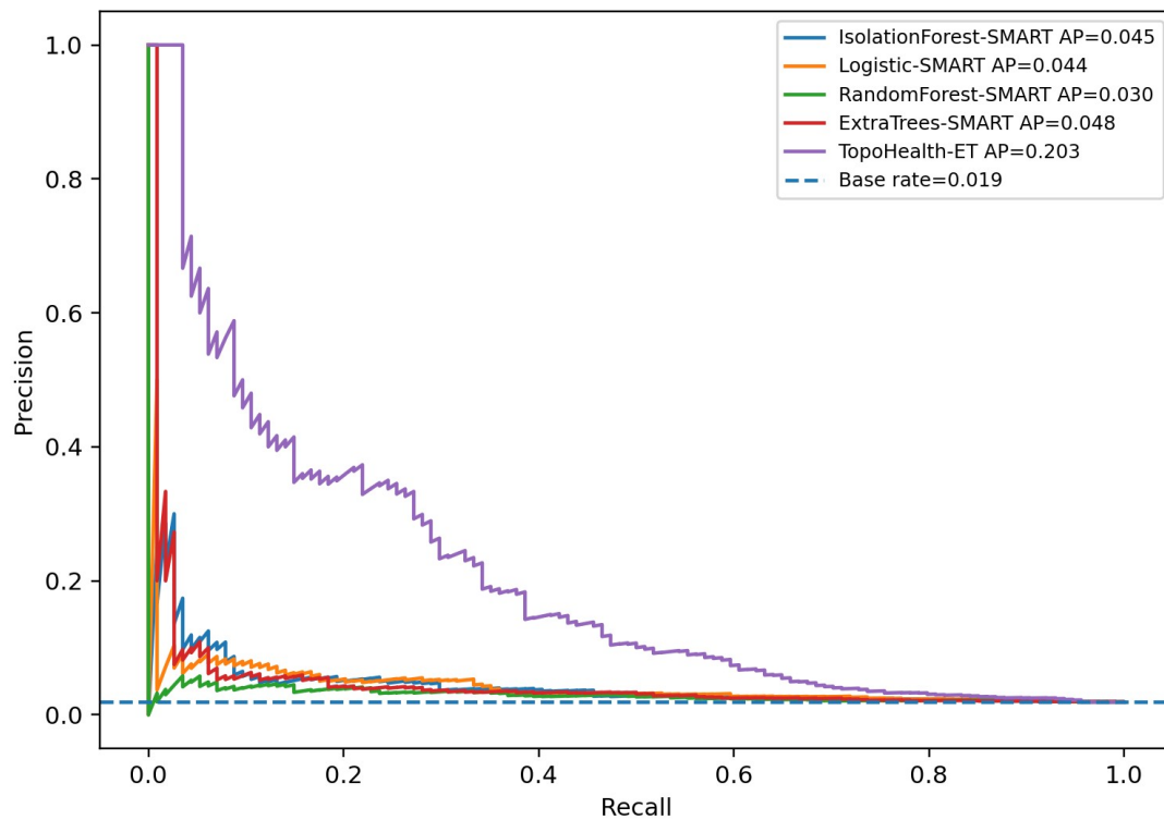
Figure 5. Precision-recall curves for principal baselines and TopoHealth-ET.
