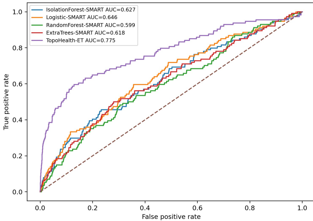
Figure 4. ROC curves for principal baselines and TopoHealth-ET on the held-out test split.
