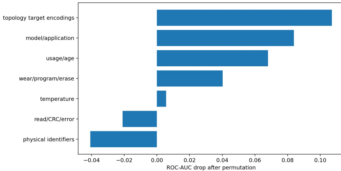
Figure 7. Grouped feature importance for the TopoHealth-ET tree component.
