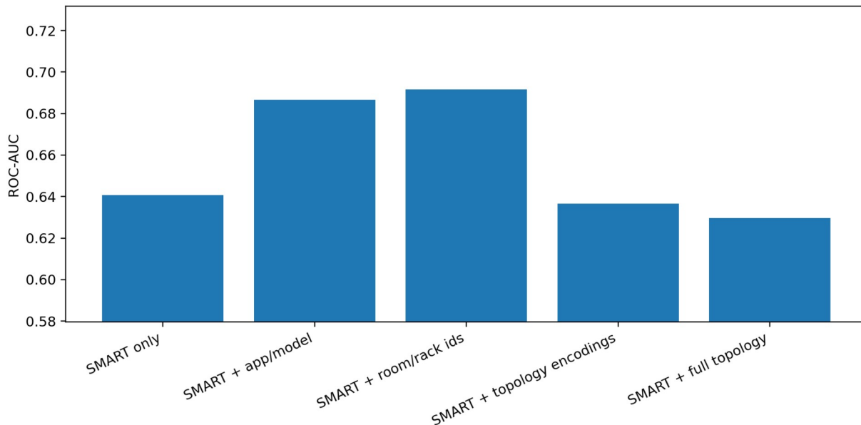
Figure 6. Ablation trend for topology-aware feature variants.
