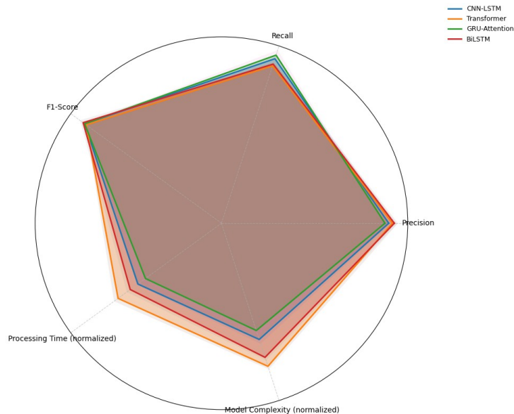
Figure 2: Multi-dimensional Architecture Performance Analysis
