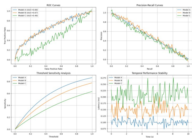
Figure 8: ROC and Precision-Recall Curves Analysis
