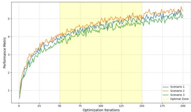
Figure 9: Optimization Convergence Analysis
