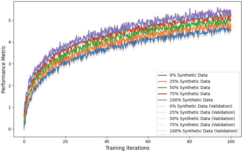
Figure 3: Learning Curves Comparison with Synthetic Data
