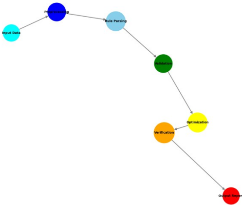
Figure 6: DRC Rule Processing Pipeline Visualization
