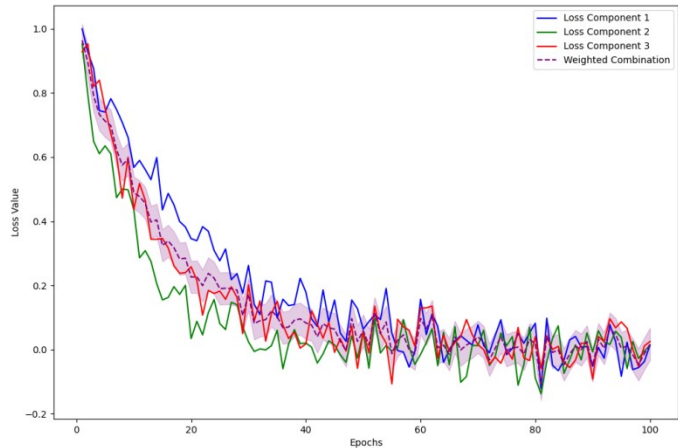
Fig. 6. Multi-Objective Loss Convergence Analysis
