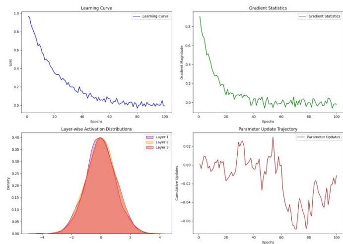
Fig. 8. Training Convergence Analysis Dashboard
