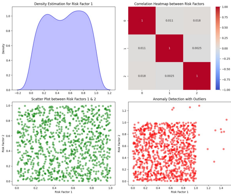
Fig. 3. Feature Distribution Analysis Framework
