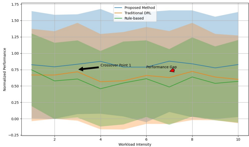
Figure 5: Performance Comparison Across Different Workload Scenarios
