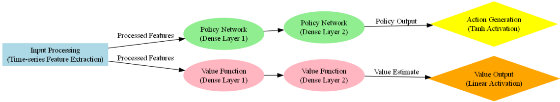
Figure 4: DRL Model Architecture for Bioprocess Optimization
