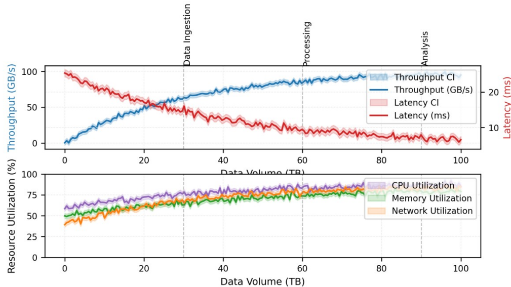
Figure 2: Data Processing Pipeline Performance
