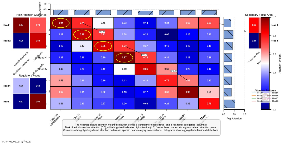
Fig. 2: Multi-Head Attention Weight Distribution Across Risk Factor Categories
