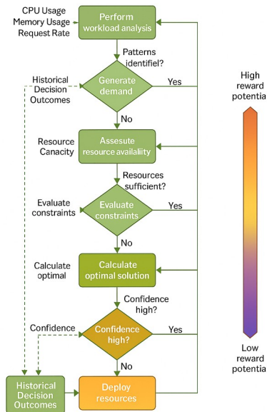
Figure 3: Decision Flow Process for Adaptive Resource Orchestration
