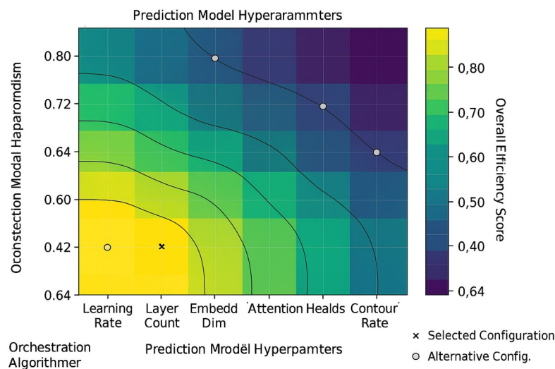
Figure 7: Hyperparameter Sensitivity Analysis for Prediction and Orchestration Components
