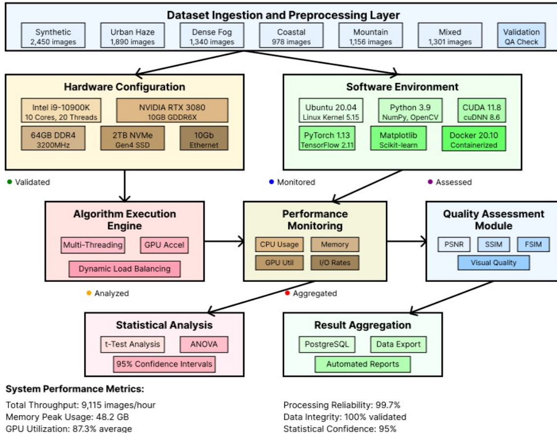
Figure 5: Experimental Framework Architecture and Validation Pipeline
