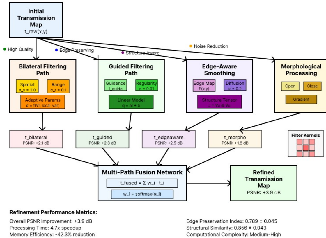
Figure 4: Multi-Stage Transmission Map Refinement Pipeline
