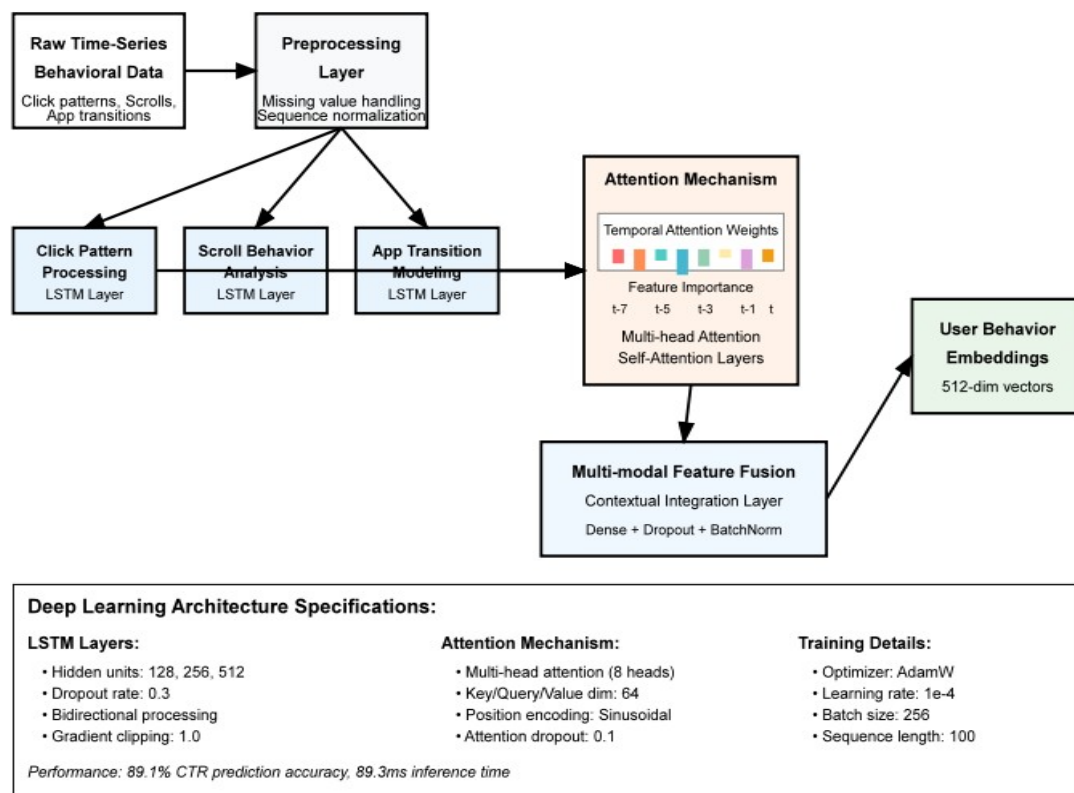
Figure 2: Temporal Behavior Pattern Recognition Using Deep Learning Architectures
