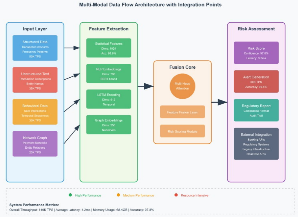
Figure 1: Multi-Modal Data Flow Architecture with Integration Points
