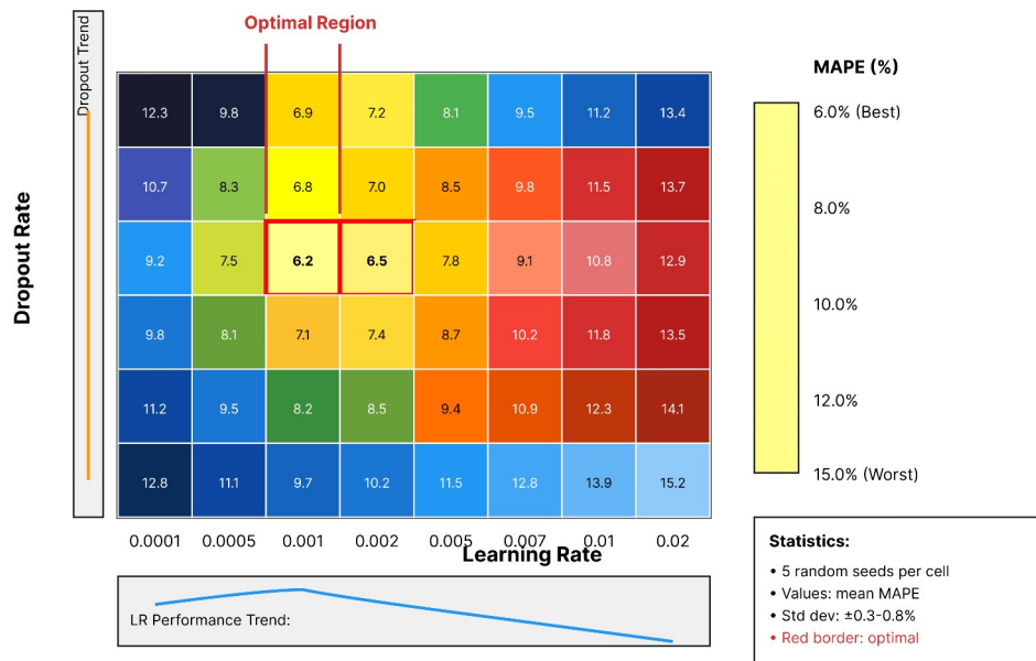
Figure 4: Parameter Sensitivity Heatmap Analysis
