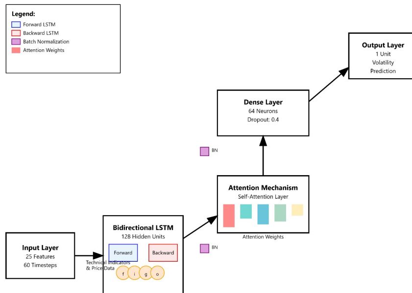
Figure 1: Enhanced LSTM Architecture with Attention Mechanism
