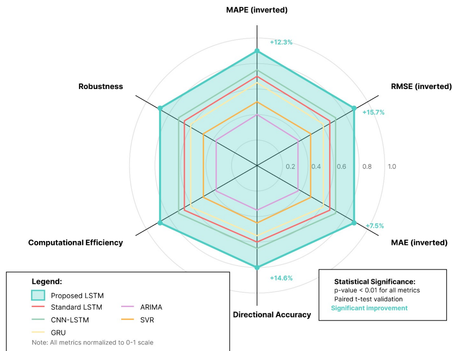
Figure 3: Performance Comparison Radar Chart
