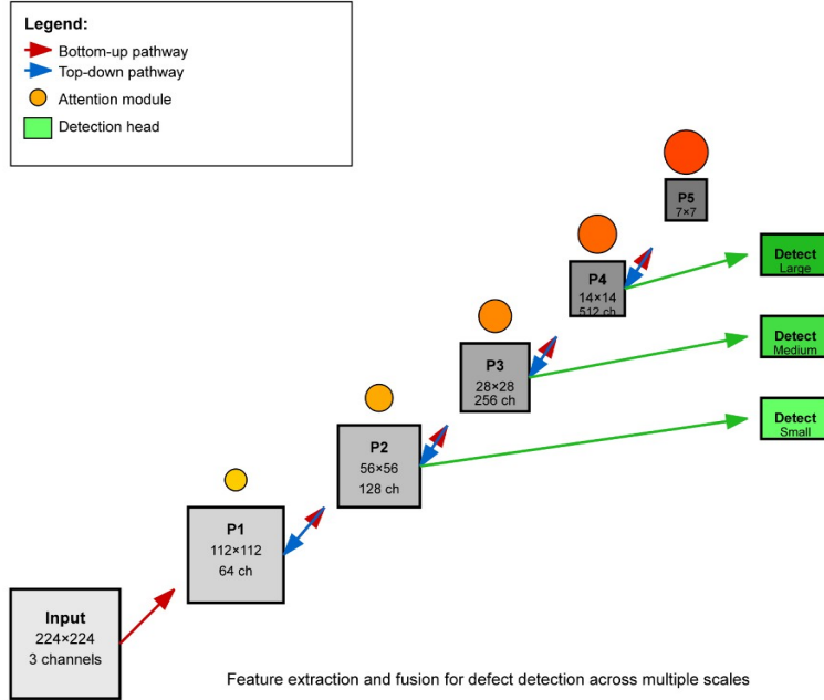
Multi-scale Feature Pyramid
