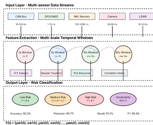
Figure 1: Multi-scale Temporal Feature Extraction Architecture
