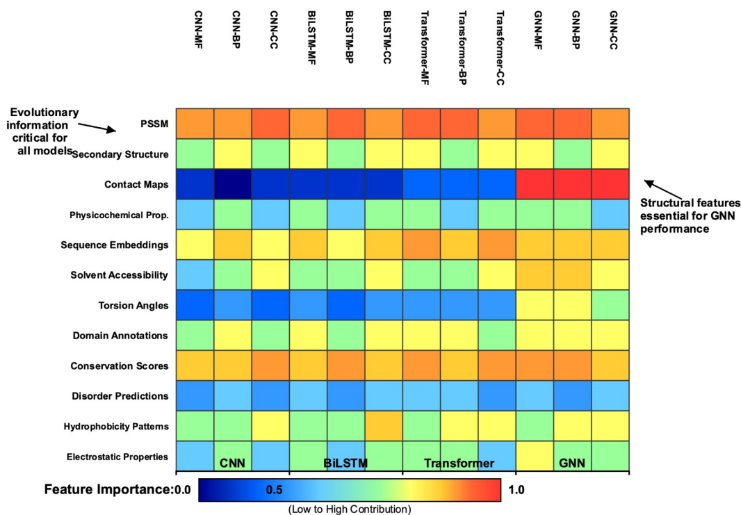
Figure 3: Feature Importance Heatmap
