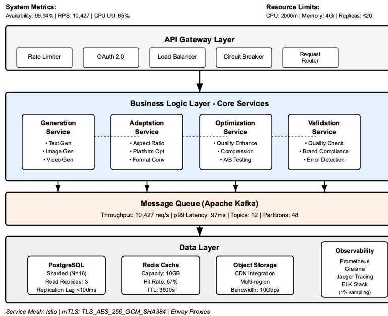
Figure 3: Microservice Architecture and Data Flow
