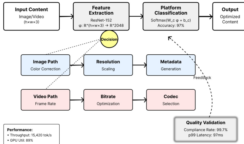
Figure 1: Platform Optimization Pipeline Architecture
