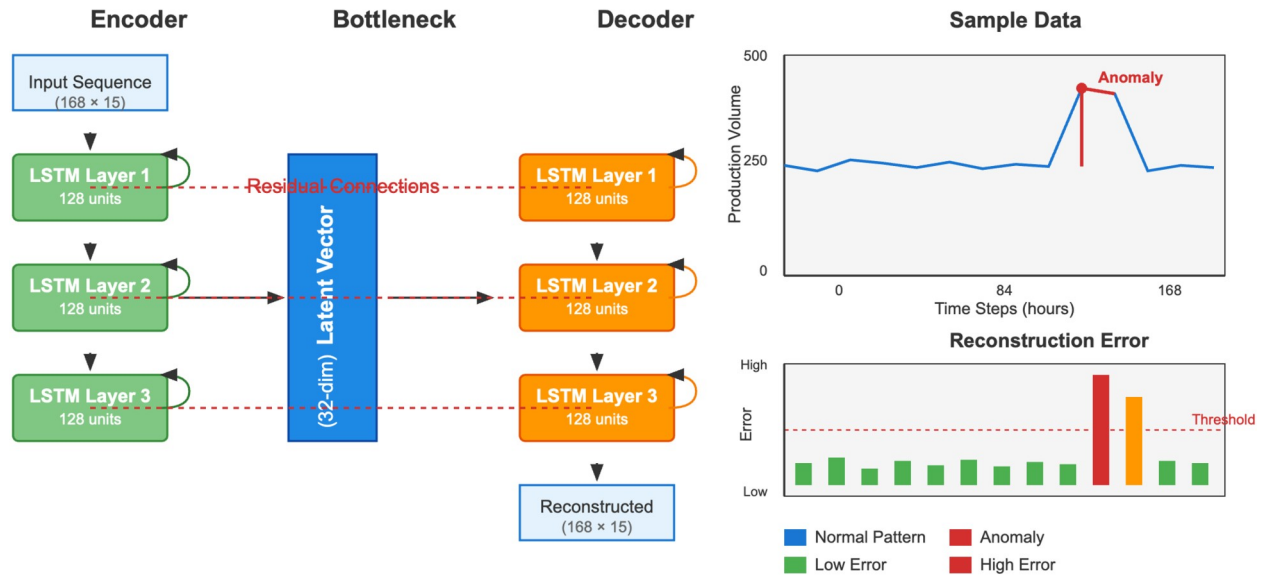
Figure 1: LSTM Autoencoder Architecture for Time Series Anomaly Detection
