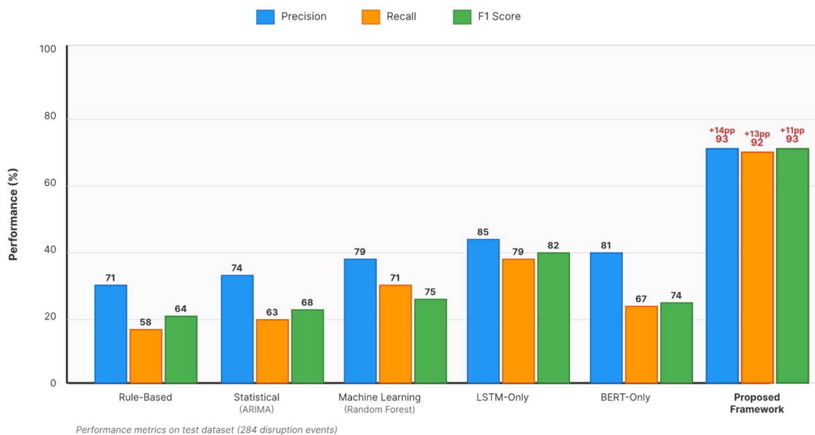
Figure 2: Detection Performance Across Baseline Methods
