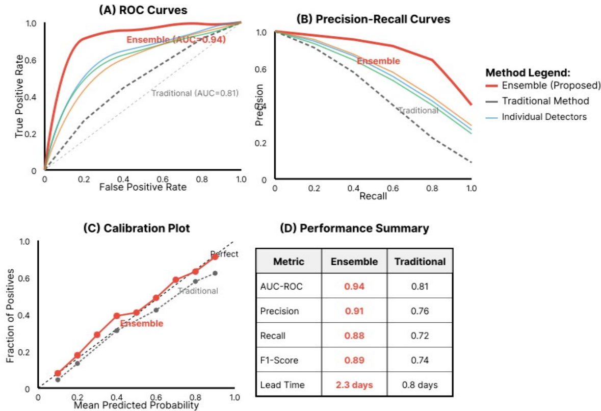
Figure 5: Comparative Performance Analysis
