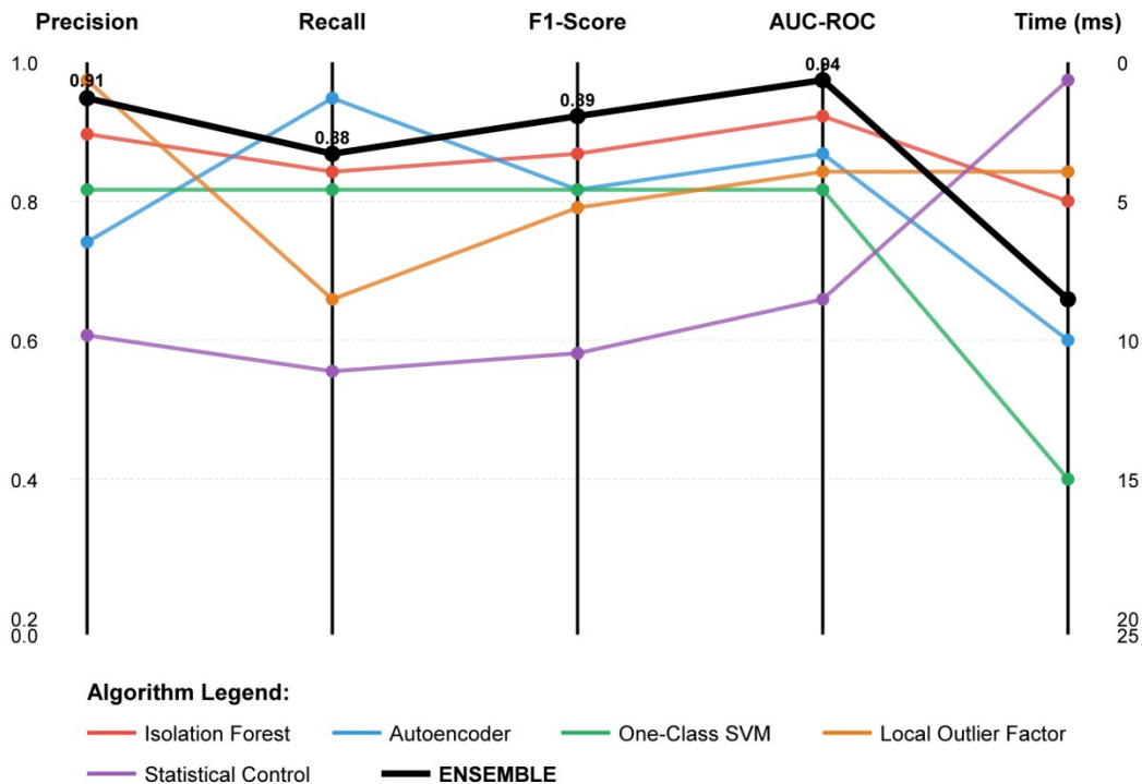
Figure 2: Ensemble Anomaly Detection Performance
