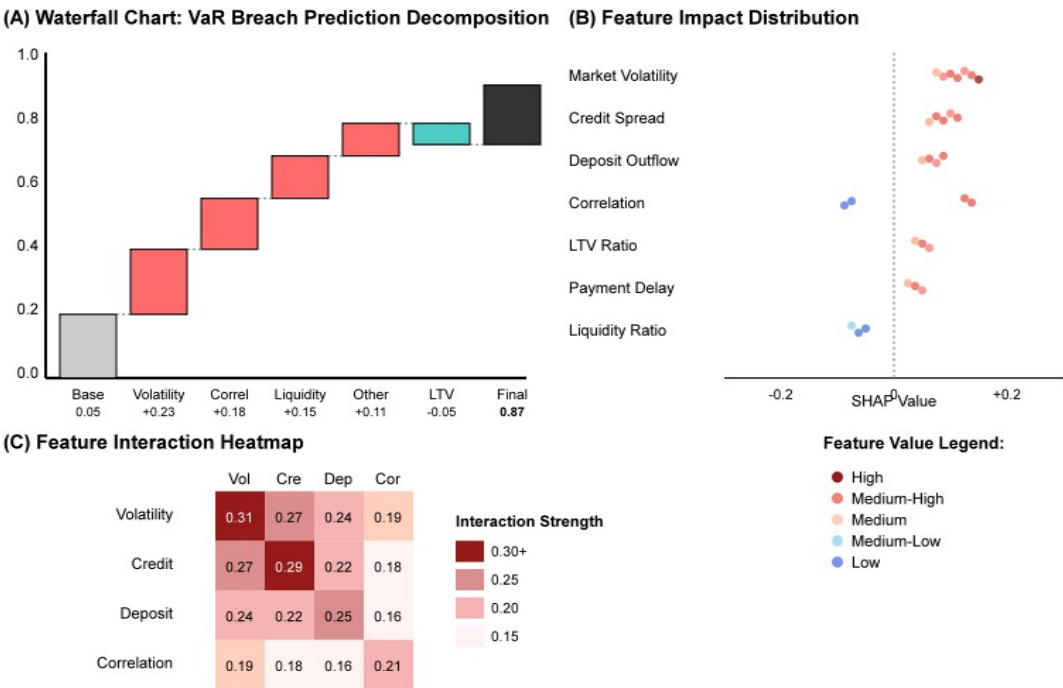
Figure 4: SHAP Value Decomposition for Risk Predictions
