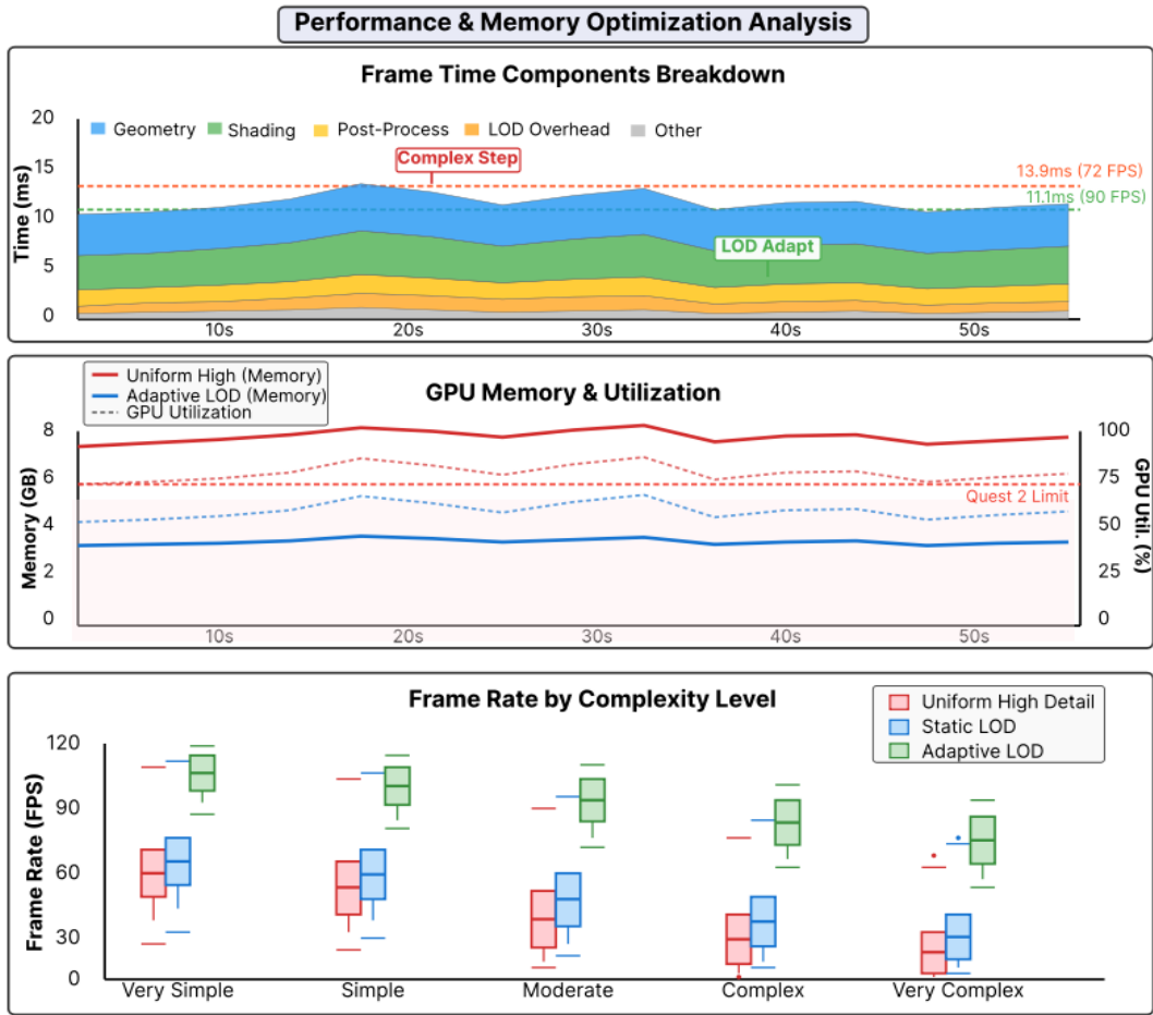
Figure 3: Memory and Performance Optimization Analysis
