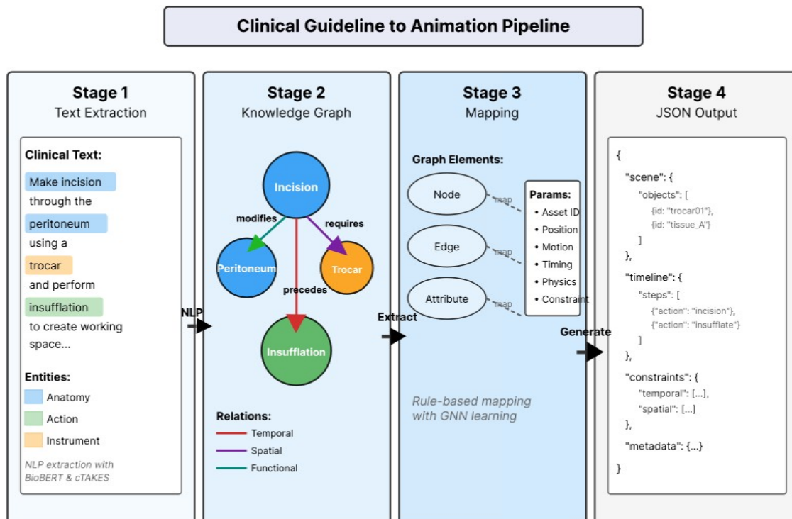
Figure 1: Knowledge Graph to Animation Specification Pipeline
