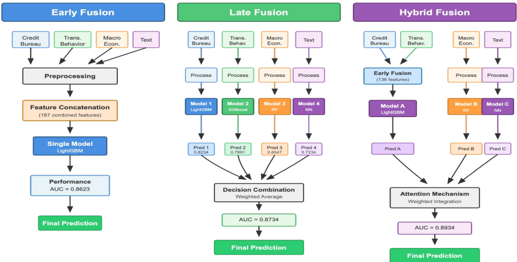
Figure 2: Fusion Strategy Comparison Workflow
