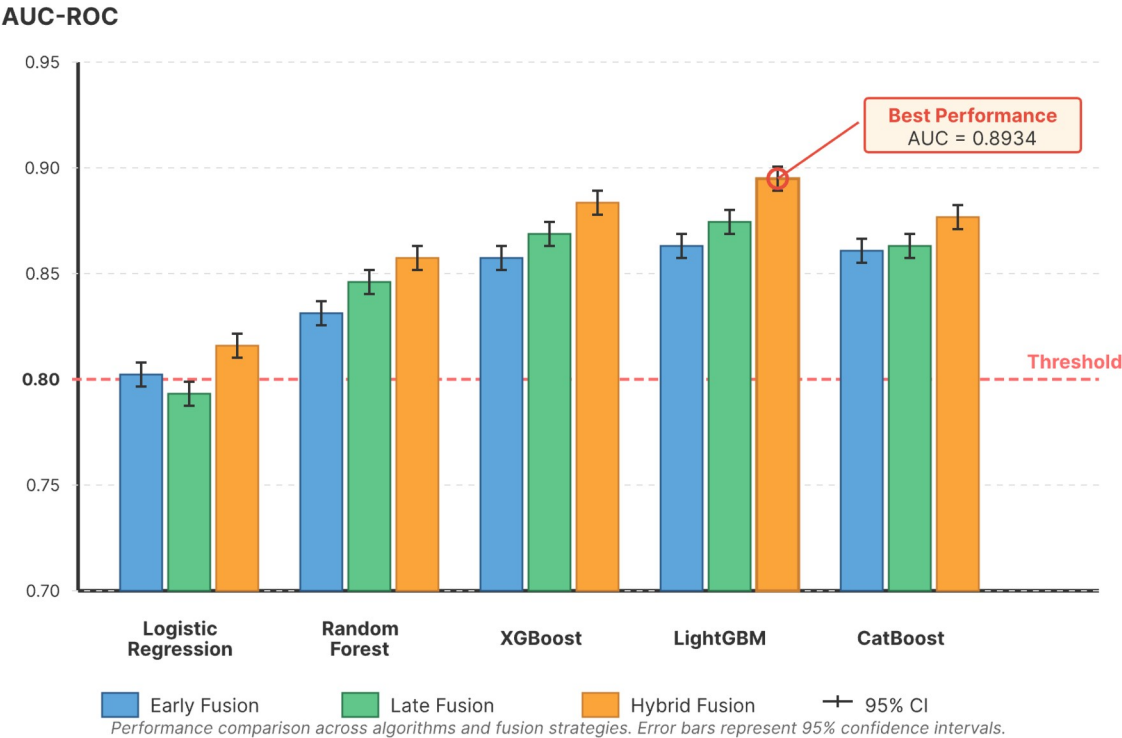
Figure 3: Algorithm Performance Comparison Across Fusion Strategies
