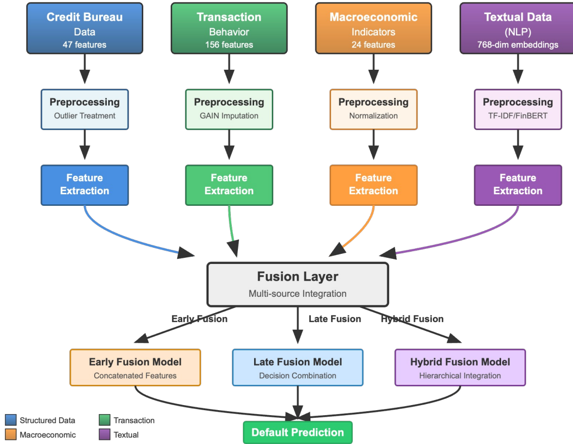
Figure 1: Multi-source Data Integration Architecture
