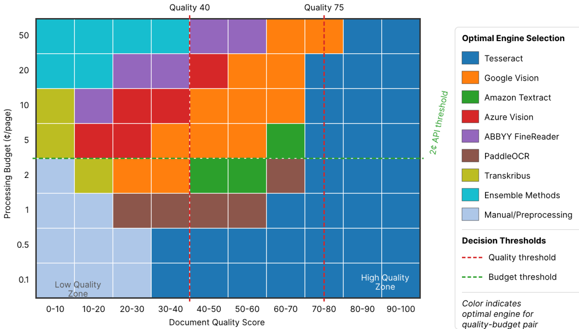
Figure 3: Heatmap Visualization of Optimal Engine Selection Across Document Quality and Processing Budget Constraints
