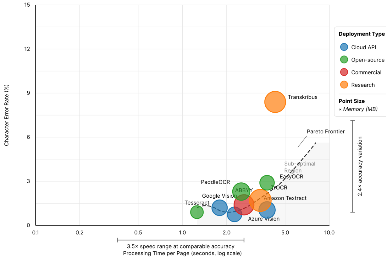
Figure 2: Scatter Plot Depicting Accuracy-Latency Pareto Frontier Across OCR Engines
