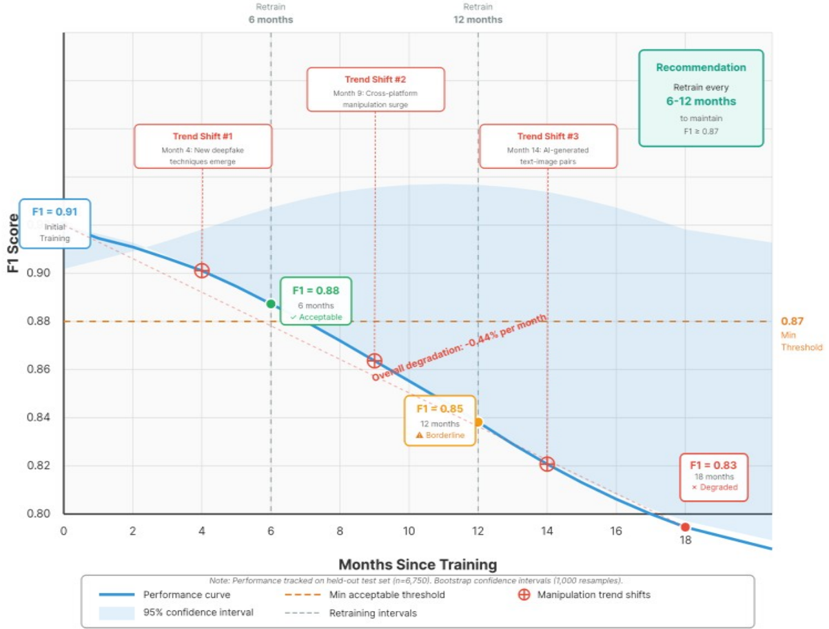
Figure 4: Temporal Generalization Analysis Over Time
