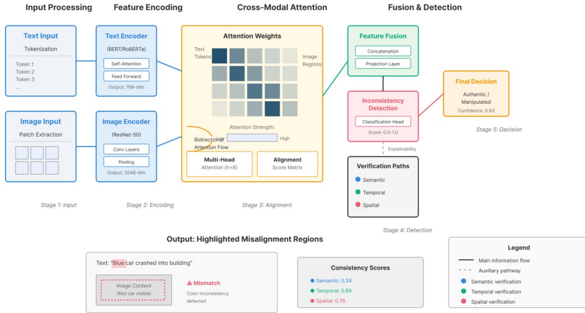
Figure 1: Cross-Modal Feature Alignment Architecture Diagram
