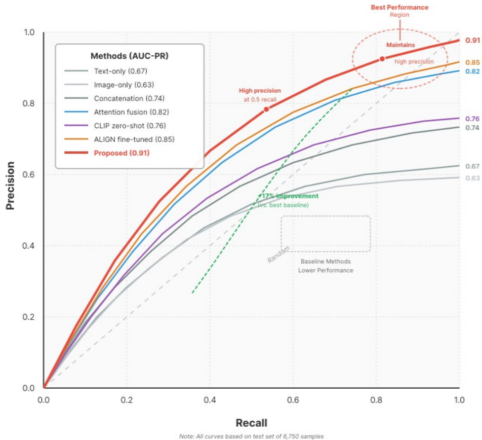
Figure 2: Precision-Recall Curves Comparing Detection Methods
