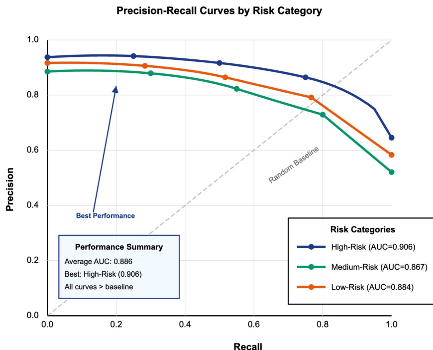
Figure 3: Precision-Recall Curves by Risk Category
