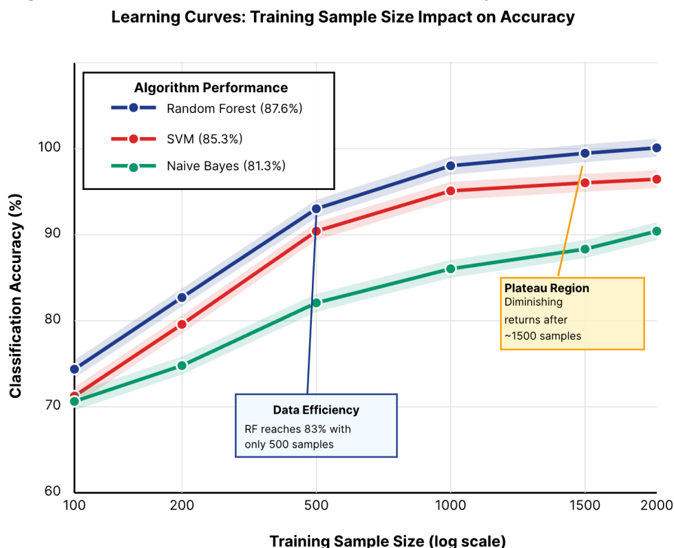
Figure 4: Training Sample Size Impact on Classification Accuracy
