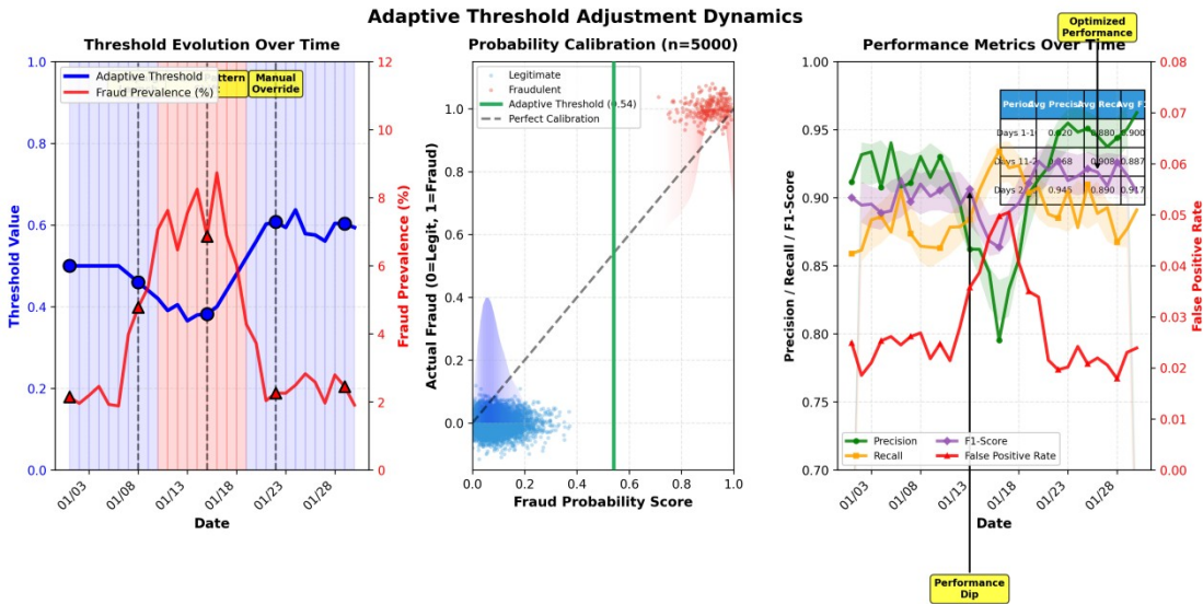
Figure 2: Adaptive Threshold Adjustment Dynamics
