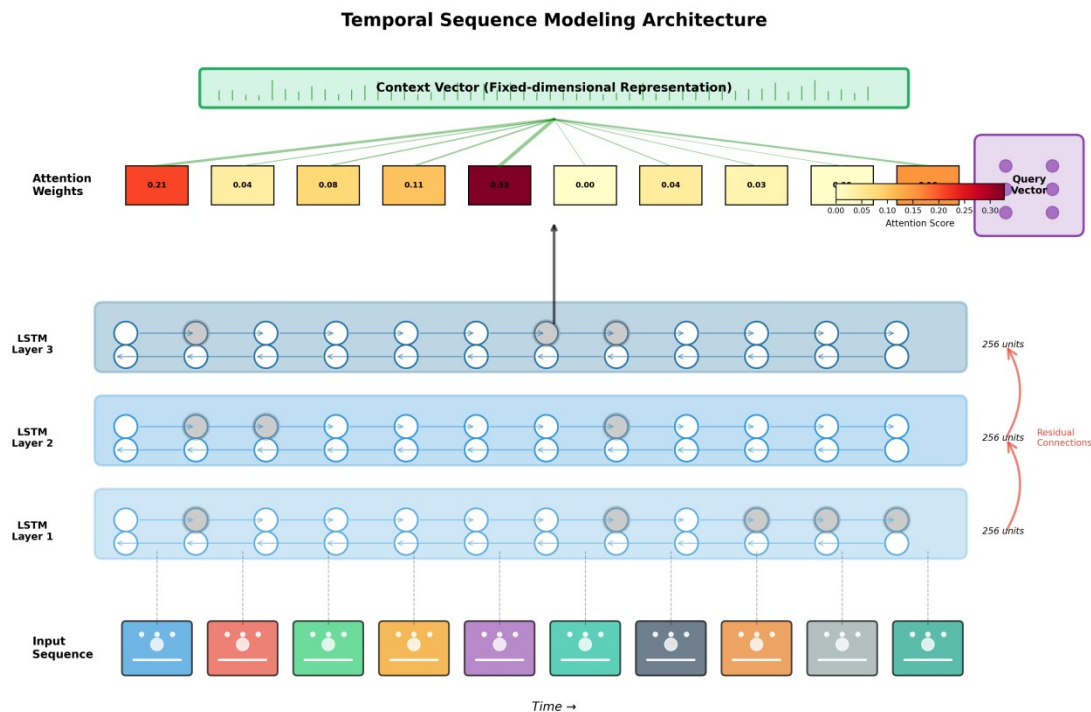
Figure 1: Temporal Sequence Modeling Architecture
