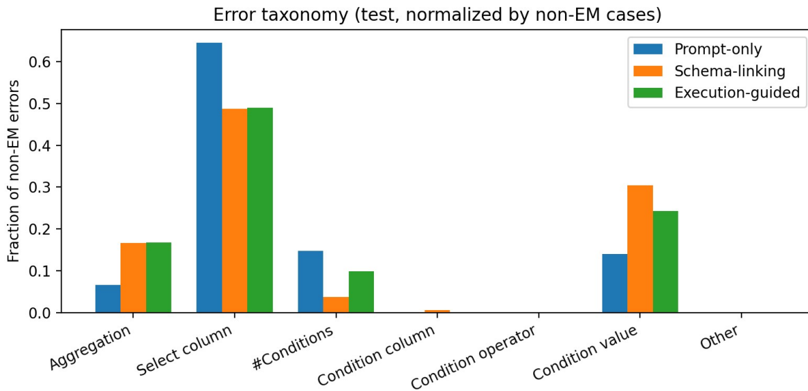
Figure 6. Normalized error taxonomy for non-EM cases (test split).
