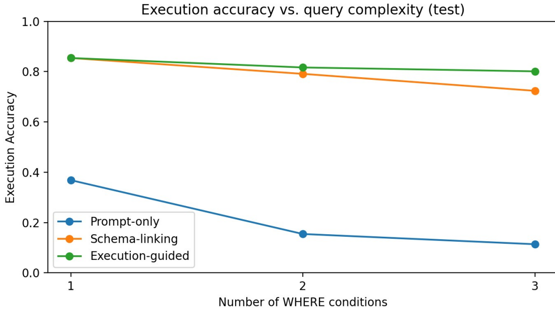
Figure 5. Execution accuracy versus number of WHERE conditions (test split).
